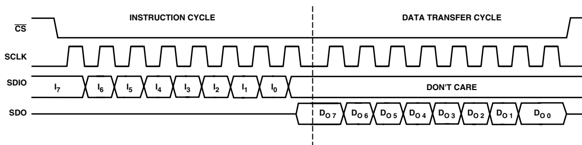
Figure 55. Three-Wire Serial Port Read Timing—Clock Stall Low
