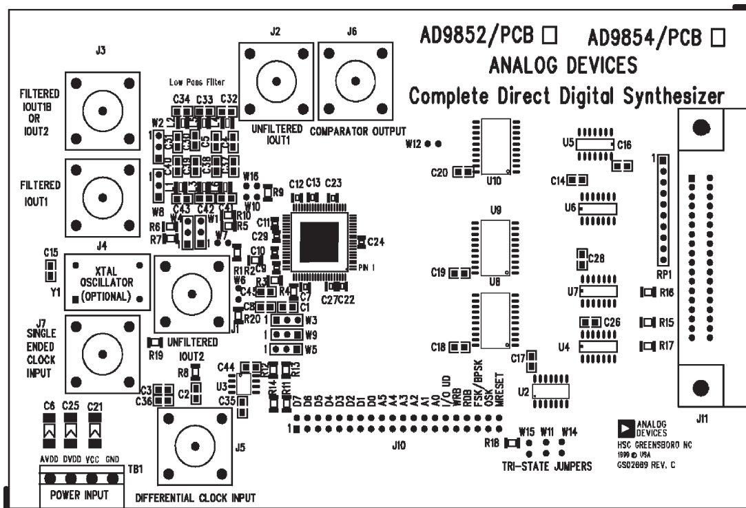
Figure 64. Assembly Drawing
