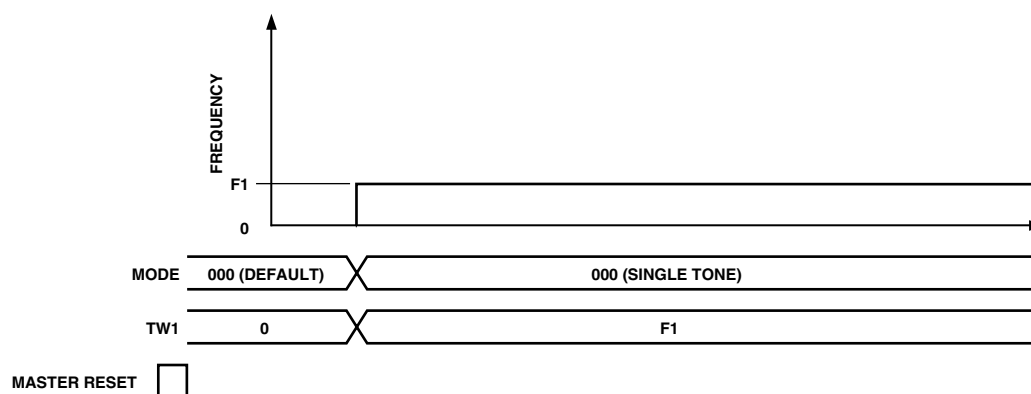
Figure 31. Default State to User-Defined Output Transition
