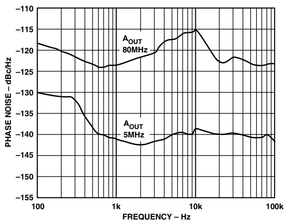
18b. Residual Phase Noise, 30 MHz REFCLK with REFCLK Multiplier = 10 \times
