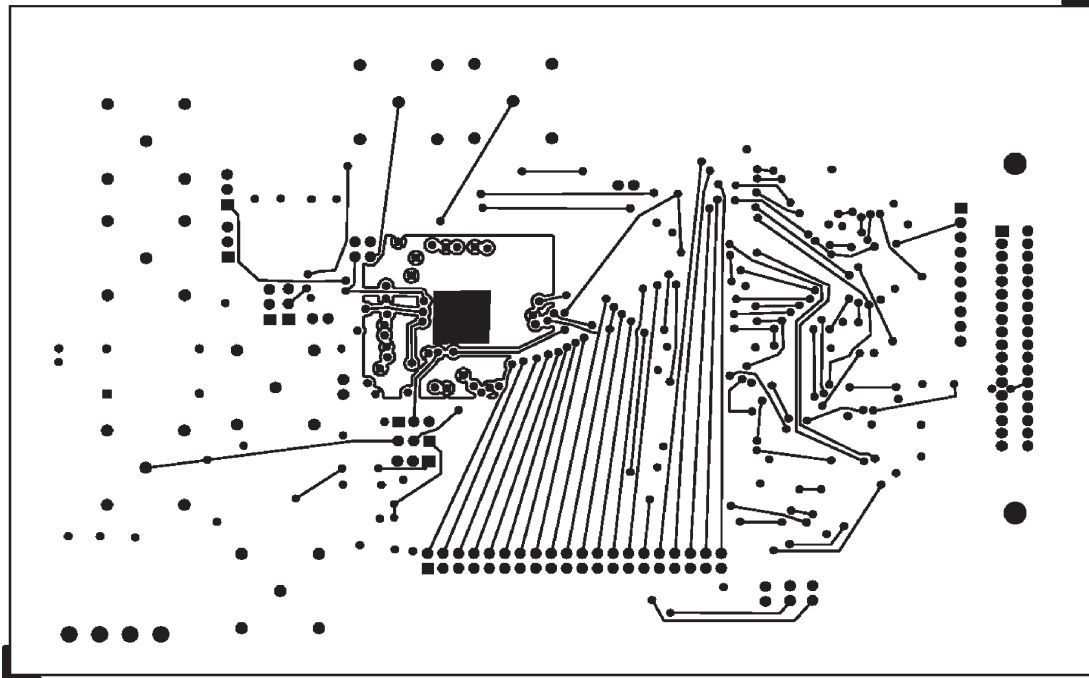
Figure 68. Bottom Routing Layer, Layer 4
