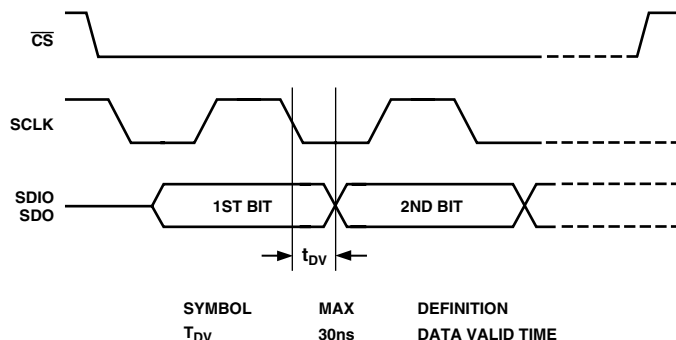
Figure 53. Timing Diagram for Read from AD9854
