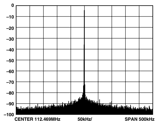
Figure 15. A slight change in tuning word yields dramatically better results. 112.469 MHz with all spurs shifted out-of-band.
