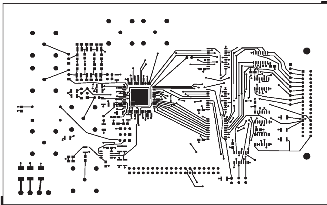
Figure 65. Top Routing Layer, Layer 1
