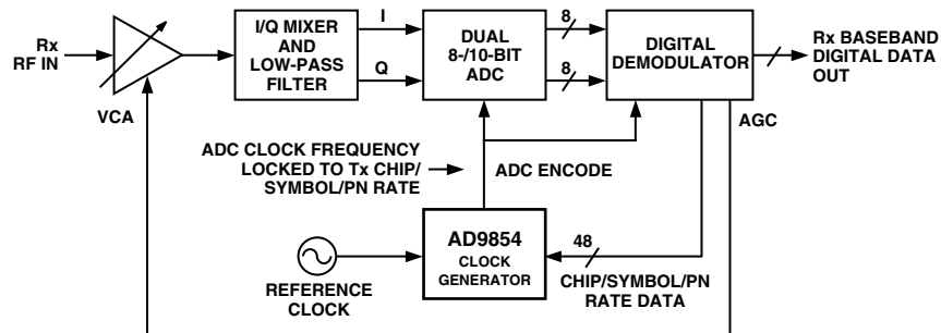
Figure 25. Chip Rate Generator in Spread Spectrum Application
