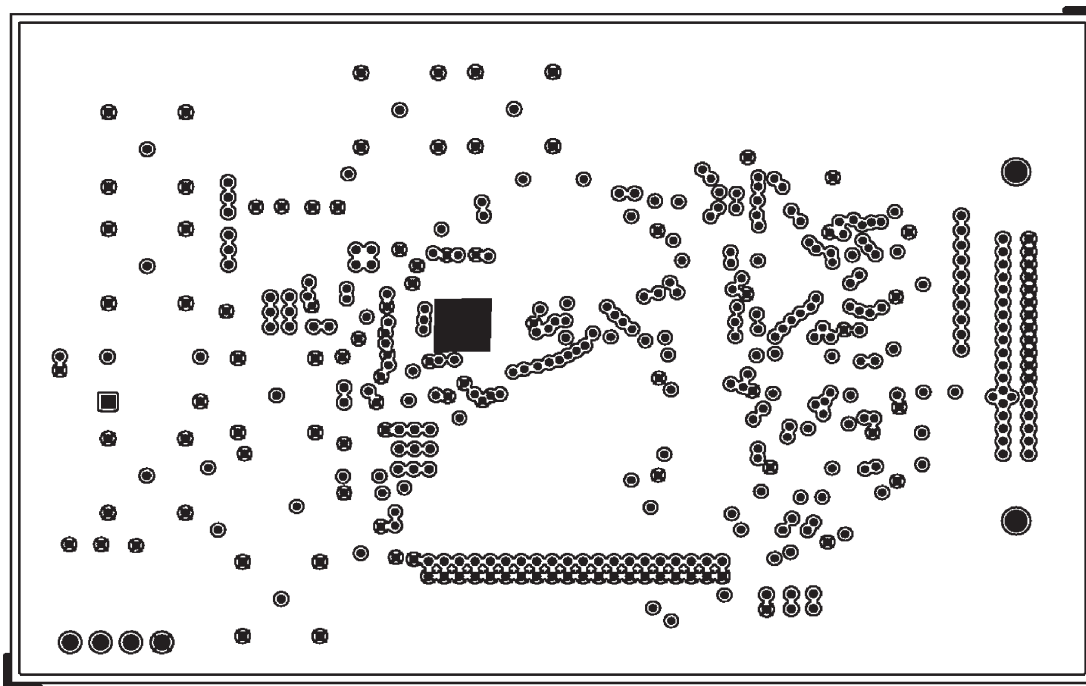
Figure 67. Ground Plane Layer, Layer 3
