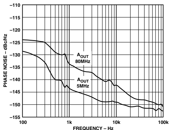
18a. Residual Phase Noise, 300 MHz REFCLK with REFCLK Multiplier Bypassed
