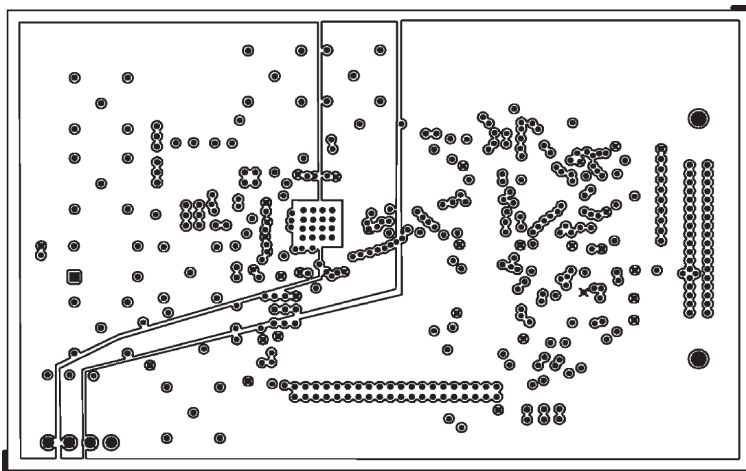
Figure 66. Power Plane Layer, Layer 2
