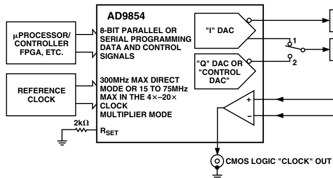
Figure 30. Frequency Agile Clock Generator Applications for the AD9854
