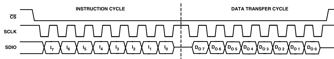
Figure 57. Two-Wire Serial Port Read Timing—Clock Stall High
