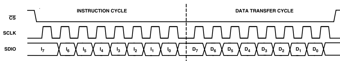
Figure 54. Serial Port Writing Timing—Clock Stall Low
