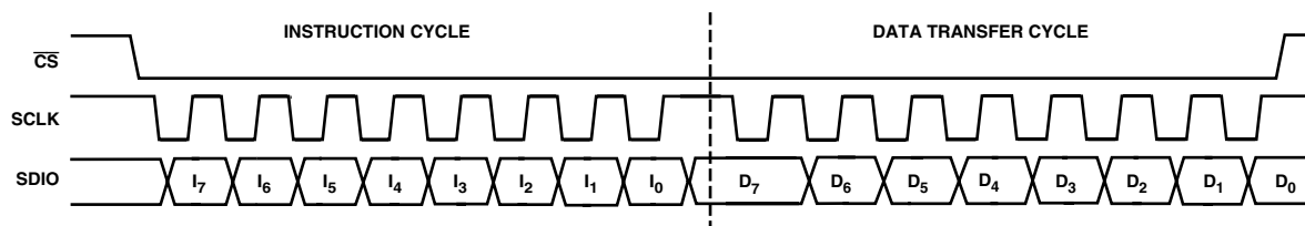
Figure 56. Serial Port Write Timing—Clock Stall High
