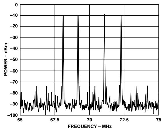
Figure 52. Spectral Plot of Four Carriers at 70MHz IF with F_{data} = 52 MSPS, PLLVDD = 0
