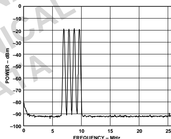
Figure 48. Spectral Plot of AD9772A Reconstructing Four GSM Modulated Carriers @ f_{DATA} = 52 MSPS, PLLVDD = 0
