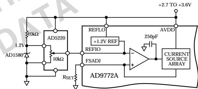
Figure 33. Single-Supply Gain Control Circuit
