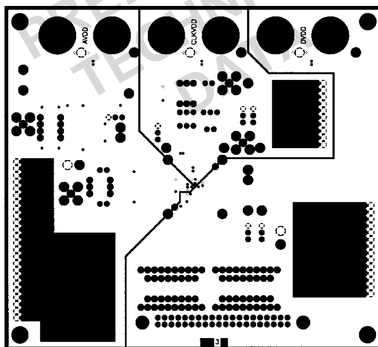
Figure 58. Power Plane PCB Layout (Layer 3)
