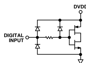
Figure 35. Equivalent Digital Input
