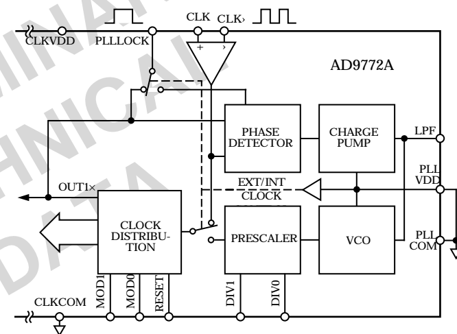
Figure 27. Clock Multiplier with PLL CLOCK Multiplier Disabled
