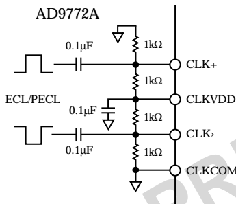
Figure 37. Differential Clock Interface
