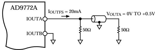
Figure 43. 0 V to +0.5 V Unbuffered Voltage Output
