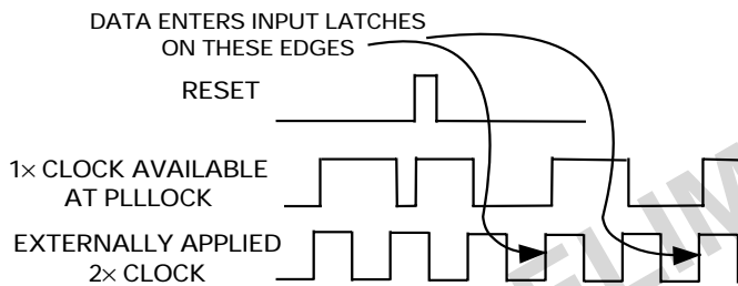
Figure 29. RESET Timing of AD9772A with PLL Disabled
