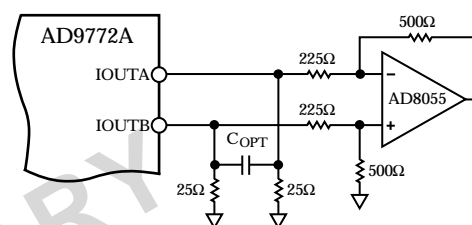
Figure 41. DC Differential Coupling Using an Op Amp
