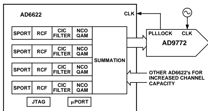
Figure 46. Generic Multicarrier Signal Chain Using the AD6622 and AD9772
