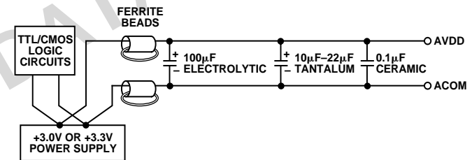
Figure 45. Differential LC Filter for +3 V or 3.3 V Applications
