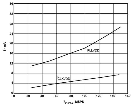
Figure 39. I_{PLLVD} and I_{CLKVDD} vs. f_{DATA}
