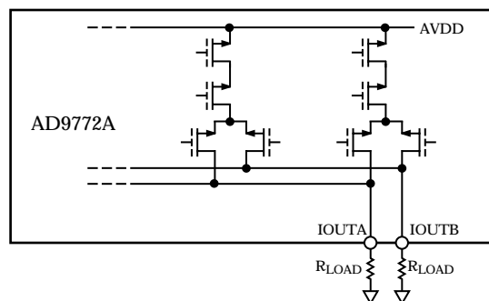
Figure 34. Equivalent Analog Output Circuit
