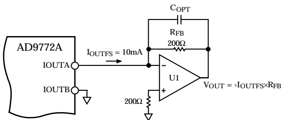
Figure 44. Unipolar Buffered Voltage Output
