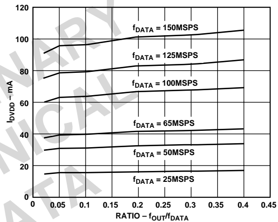
Figure 38. I_{DVDD} vs. Ratio @DVDD=3.3V
