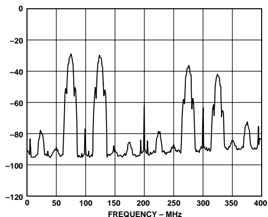
Figure 50. Spectral Plot of 16-QAM Signal in Direct IF Mode at f_{DATA} = 100 MSPS
