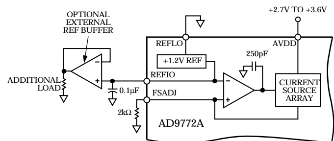
Figure 30. Block Diagram of Internal DAC, 1.2 V Reference, and Reference Control Circuits
