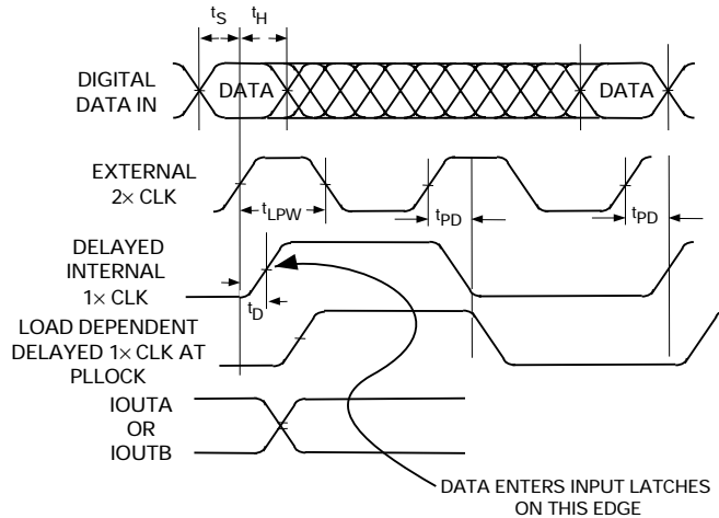
Figure 28. Internal Timing of AD9772A with PLL Disabled
