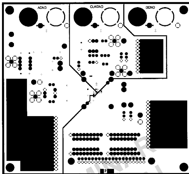
Figure 57. Ground Plane PCB Layout (Layer 2)
