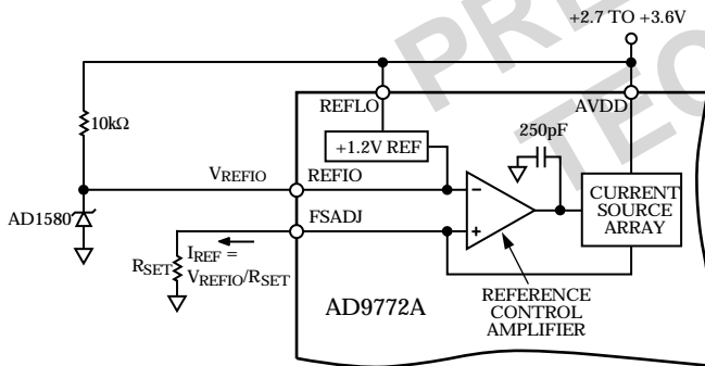
Figure 31. Internal Reference Configuration
