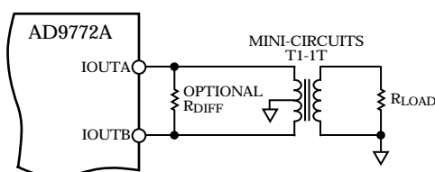
Figure 40. Differential Output Using a Transformer
