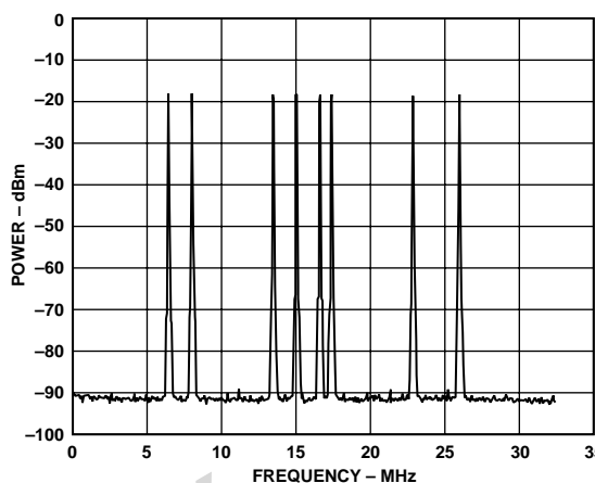
Figure 47. Spectral Plot of AD9772A Reconstructing Eight IS-136 Modulated Carriers @ f_{DATA} = 64.54 MSPS, PLLVDD = 0
