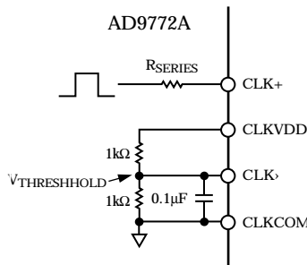
Figure 36. Single-Ended Clock Interface
