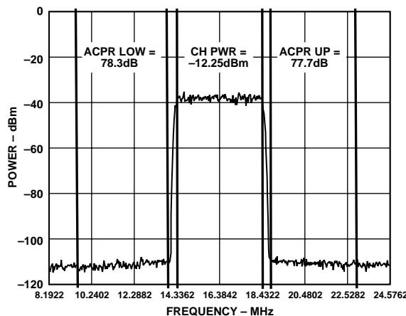
Figure 49. AD9772A Achieves 78 dB ACPR Performance Reconstructing a "WCDMA-Like" Test Vector with f_{\text{DATA}} = 65.536 \text{ MSPS} and \text{PLLVD} = 0 \text{ Volts}
