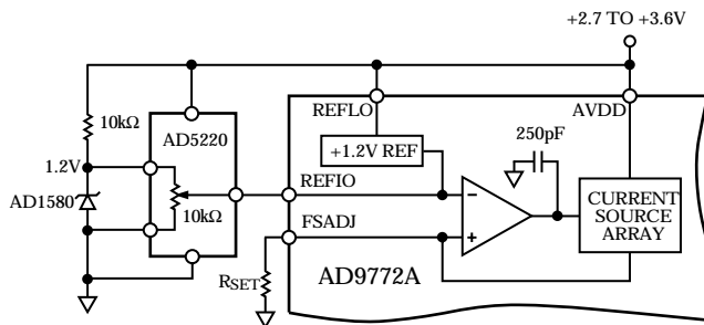
Figure 32. External Reference Configuration
