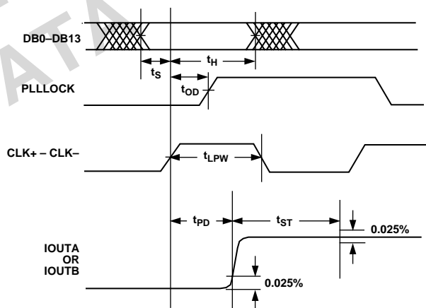
Figure 1b. Timing Diagram—PLL Clock Multiplier Disabled
