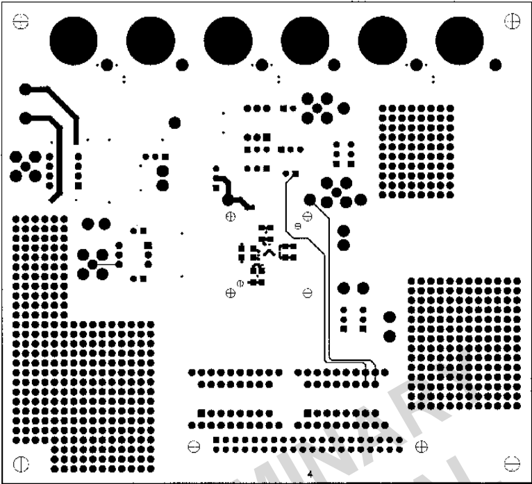
Figure 59. Solder Side PCB Layout (Layer 4)
