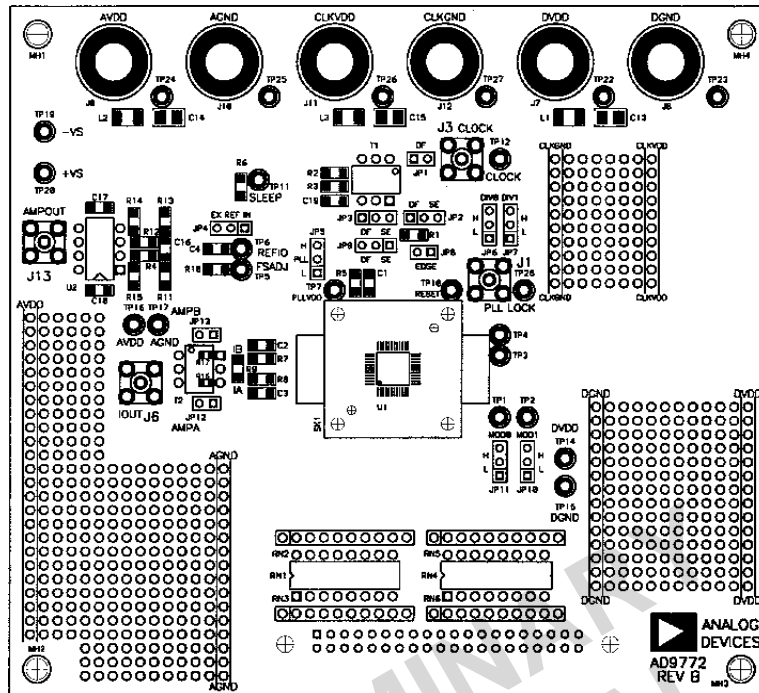
Figure 55. Silkscreen Layer-Top
