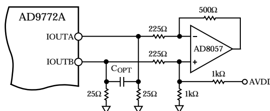
Figure 42. Single Supply DC Differential Coupled Circuit
