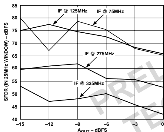
Figure 51. Dual Tone "Windowed" SFDR vs. A_{OUT} at f_{DATA} = 100 MSPS
