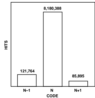
Figure 4. "Grounded-Input" Histogram (Input Span = 2 V p-p)
