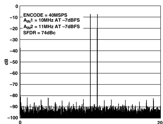
TPC 17. Two-Tone Intermodulation Distortion (10 MHz, 11 MHz; 1 V p-p, FS = 40 MSPS)
