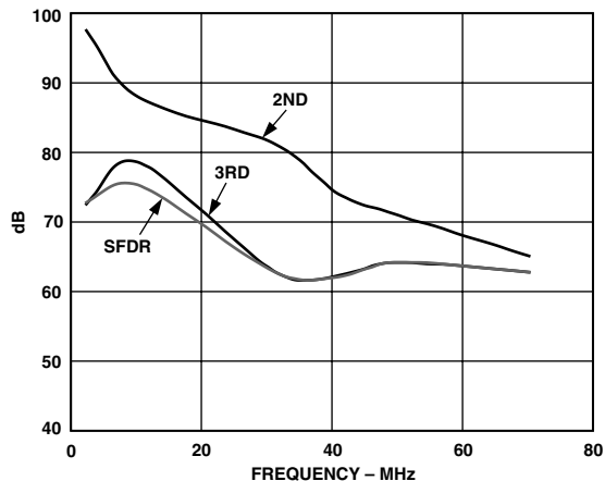
TPC 7. Harmonic Distortion (Second and Third) and SFDR vs. A_{IN} Frequency (1 V p-p and 2 V p-p, f_s = 65 MSPS)
