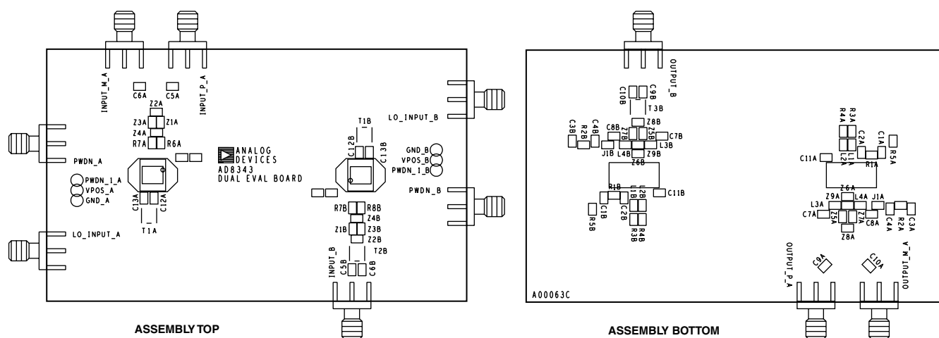
Figure 25. Evaluation Board Assembly Drawing
