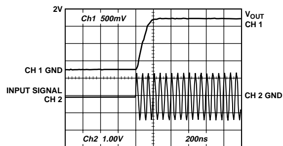
Figure 16. V_{OUT} Rise Time
