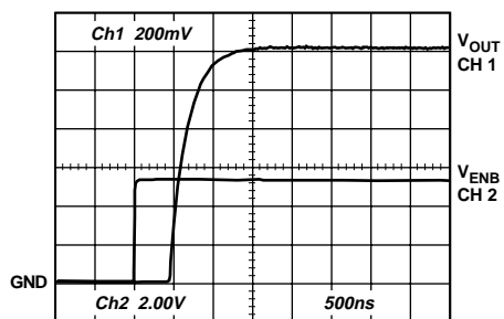
Figure 13. Power-Up Response Time
