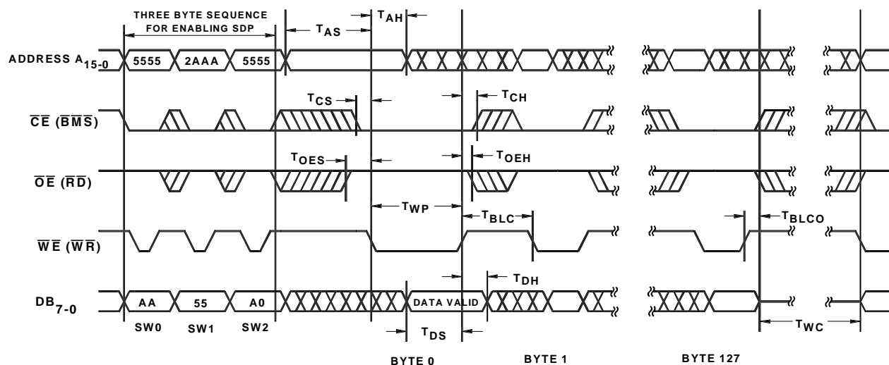
Figure 22. \overline{WR} Controlled Page Mode Write Cycle Timing
