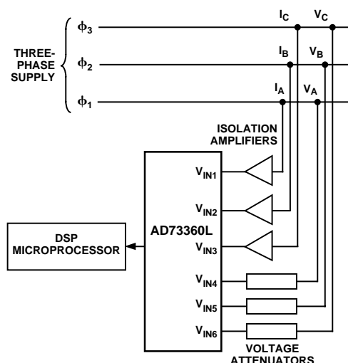
Figure 31. Three-Phase Power Metering
