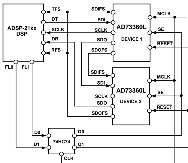
Figure 17. Connection of Two AD73360Ls Cascaded to ADSP-21xx
