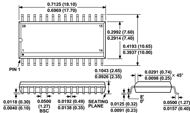
Small Outline IC (SOIC) (R-28)
