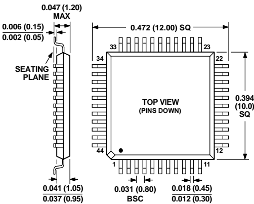
44-Lead Thin Quad Flatpack (SU-44)
