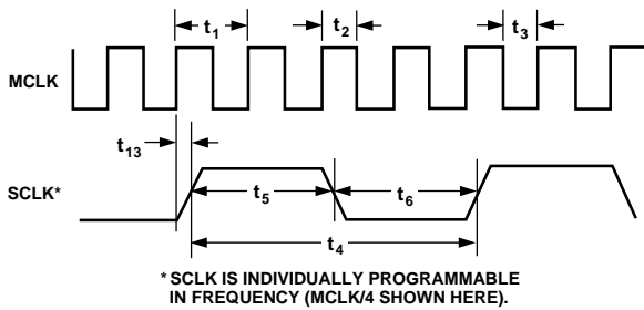
Figure 3. SCLK Timing
