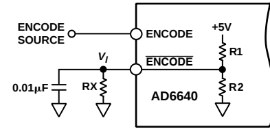
Figure 26. Lower Logic Threshold for Encode
