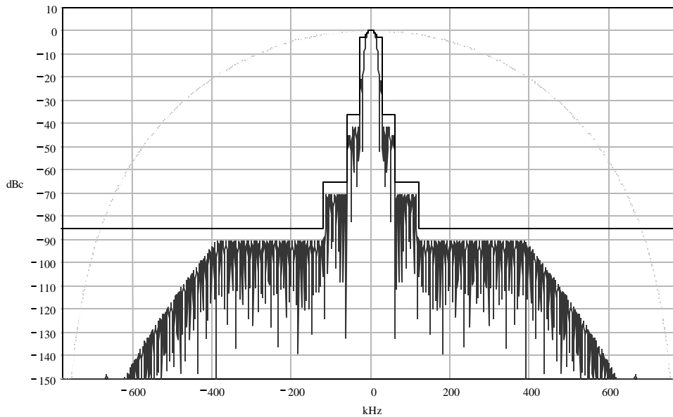
Figure 21. The filter above is designed to meet the IS-136 specifications. For this configuration, the clock is set to 61.44 MSPS with a total decimation rate of 320 providing an output data rate of 194.4 kSPS or 4 samples per symbol.
