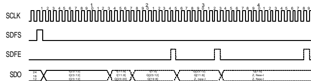
Figure 30. SDFS Valid for One SCLK Cycle
