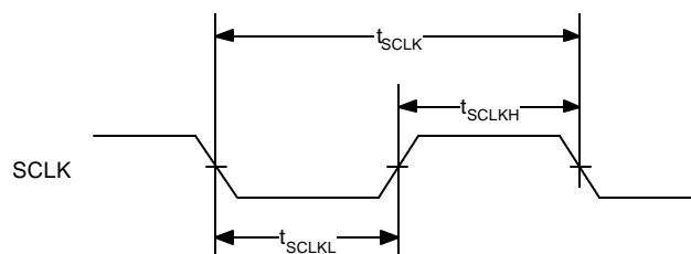
Figure 38. SCLK Timing Requirements
