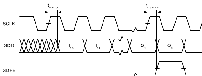
Figure 45. SDO, SDFE Switching Characteristics
