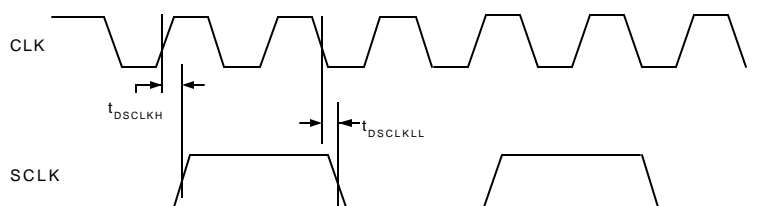
Figure 8. SCLK Switching Characteristics (Divide by 3 or ODD integer)
