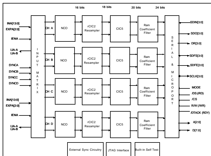
Figure 1. AD6624 Block Diagram
