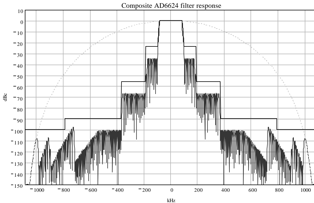
Figure 2b. Composite Filter Response of rCIC2 , CIC5 , and RCF
