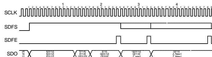
Figure 31. SDFS is High During Data Shift
