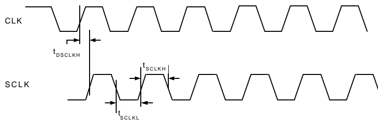
Figure 6. SCLK Switching Characteristics (Divide by 1)
