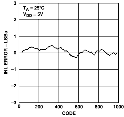
TPC 2. AD5317 Typical INL Plot
