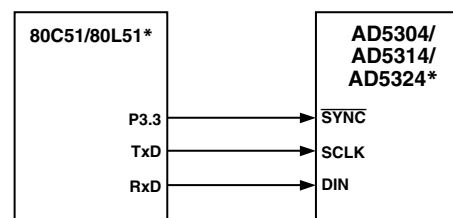
Figure 35. AD5304/AD5314/AD5324 to 80C51/80L51 Interface
