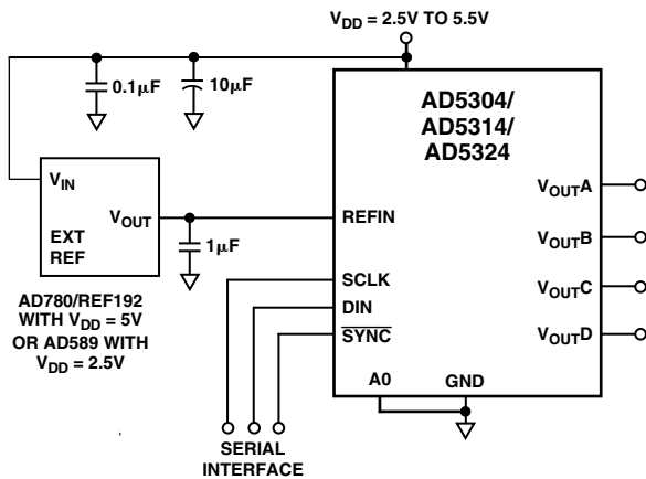
Figure 37. AD5304/AD5314/AD5324 Using External Reference
