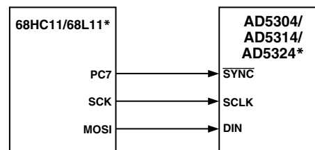
Figure 34. AD5304/AD5314/AD5324 to 68HC11/68L11 Interface
