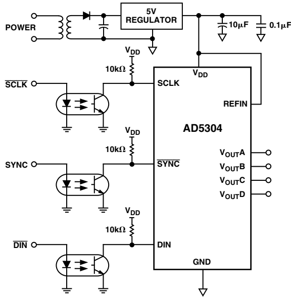
Figure 39. AD5304 in an Opto-Isolated Interface
