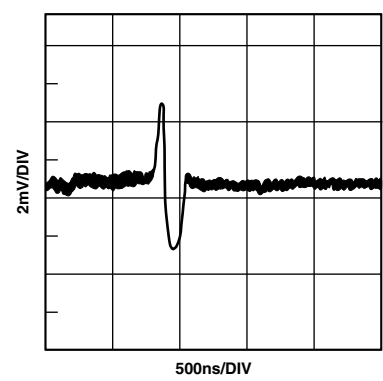
Figure 25. DAC-DAC Crosstalk
