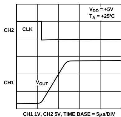
Figure 19. Half-Scale Settling (1/4 to 3/4 Scale Code Change)
