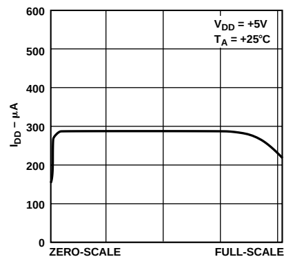
Figure 15. Supply Current vs. Code
