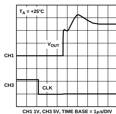
Figure 21. Exiting Power-Down to Midscale
