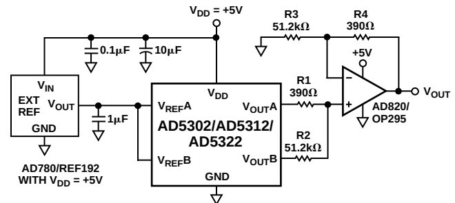
Figure 42. Coarse/Fine Adjustment
