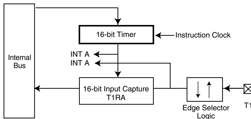
Figure 16: Input Capture Mode
