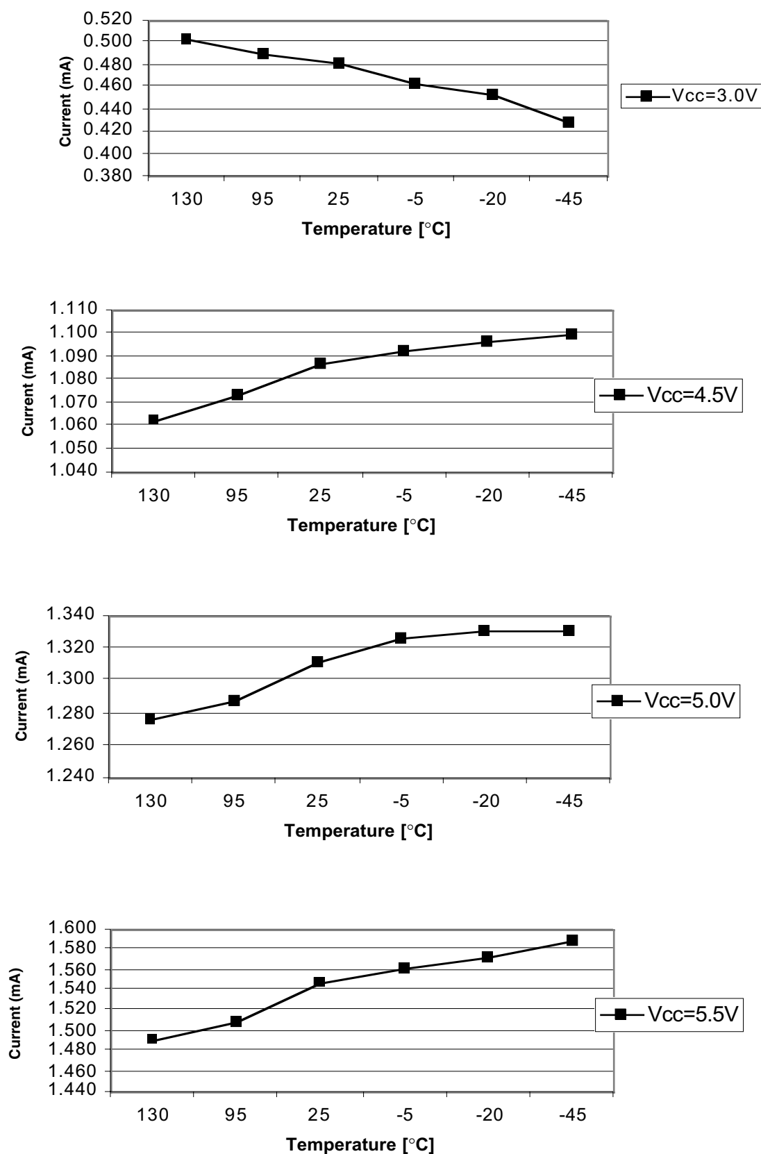
Figure 6: I_{CC} Active
