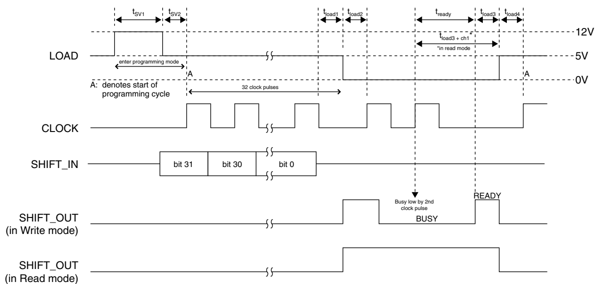
Figure 23 - Programming Protocol
