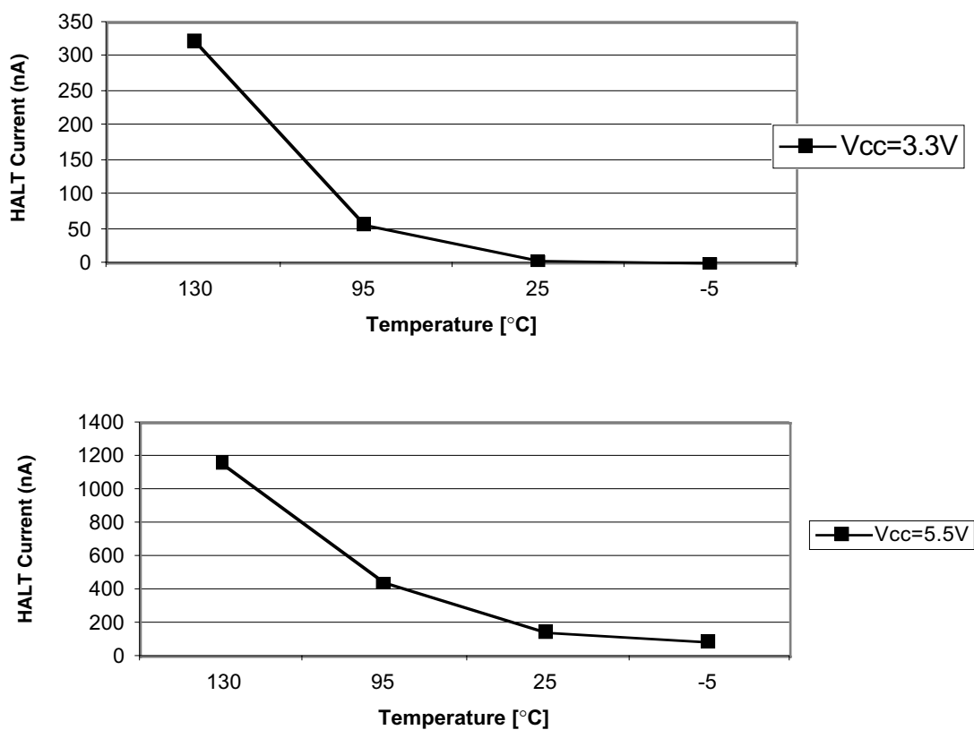
Figure 7: HALT Current
