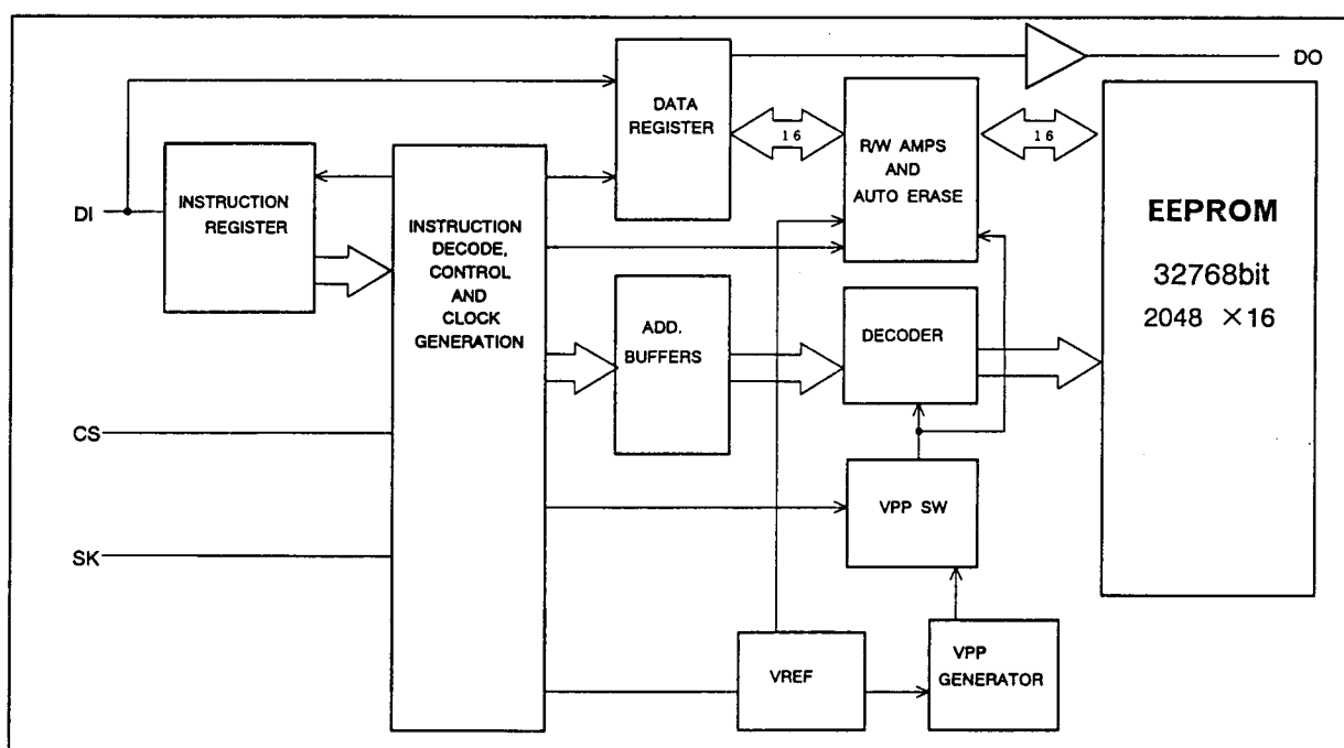
Block Diagram
