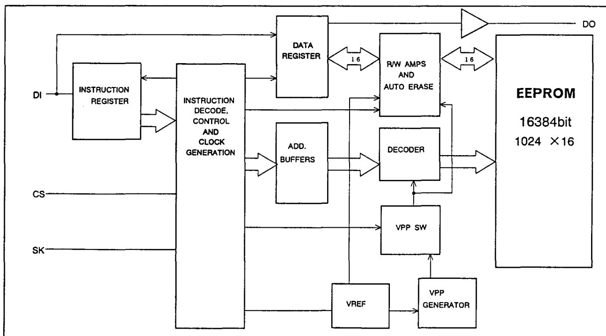
Block Diagram
