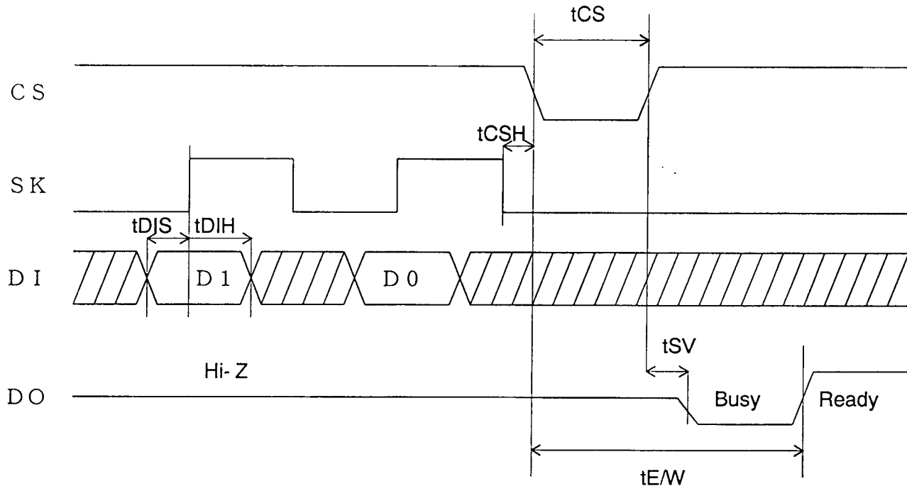
Busy/Ready Signal Output
