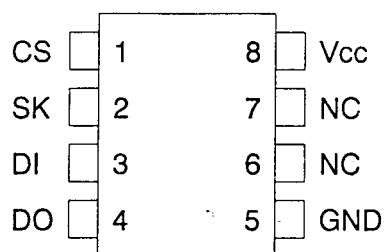
8pinDIP
