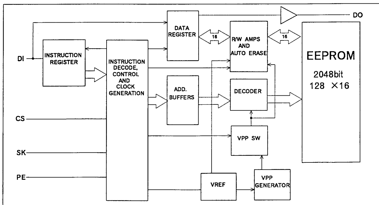
Block Diagram
