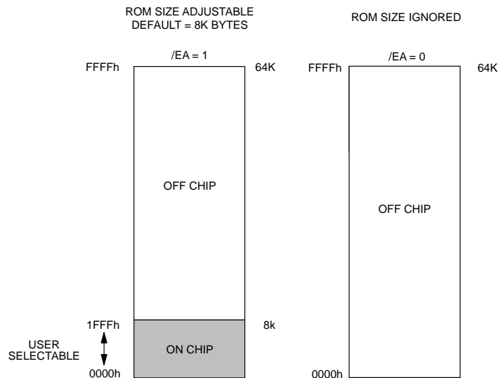
ROM MEMORY MAP Figure 2
