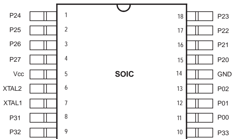
Figure 3. 18-Pin SOIC
