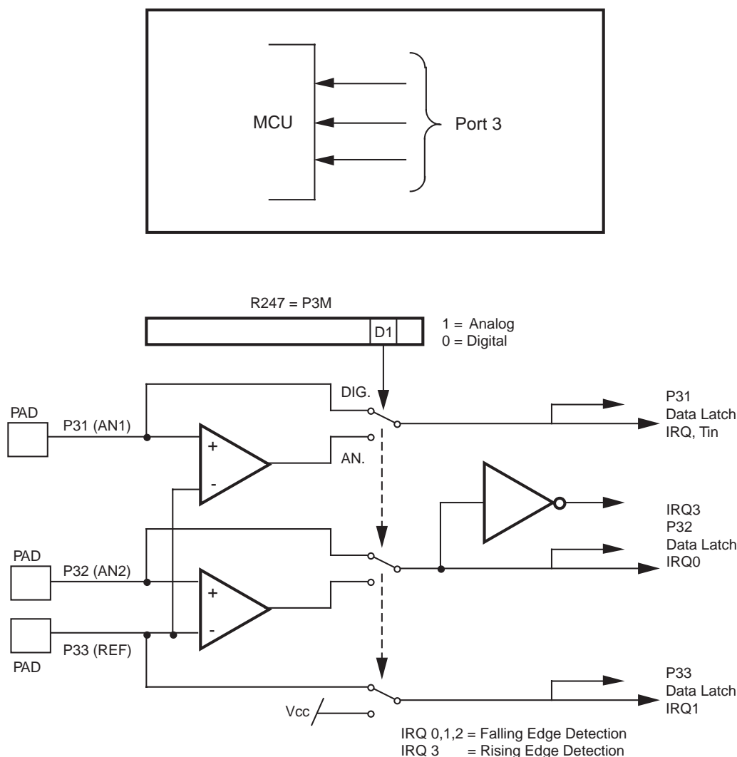
Figure 8. Port 3 Configuration
