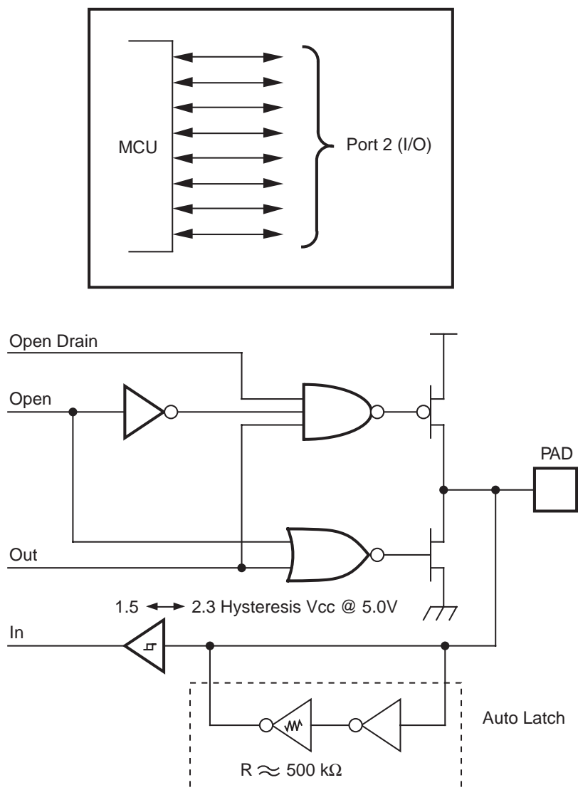
Figure 7. Port 2 Configuration
