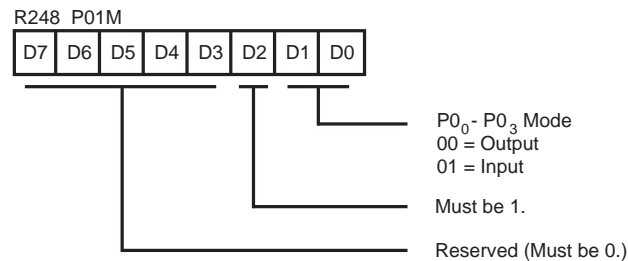
Figure 24. Port 0 and 1 Mode Register (F8 H : Write Only)
