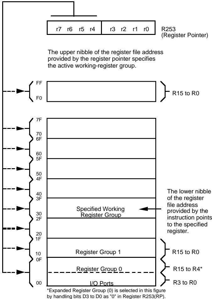
Figure 12. Register Pointer
