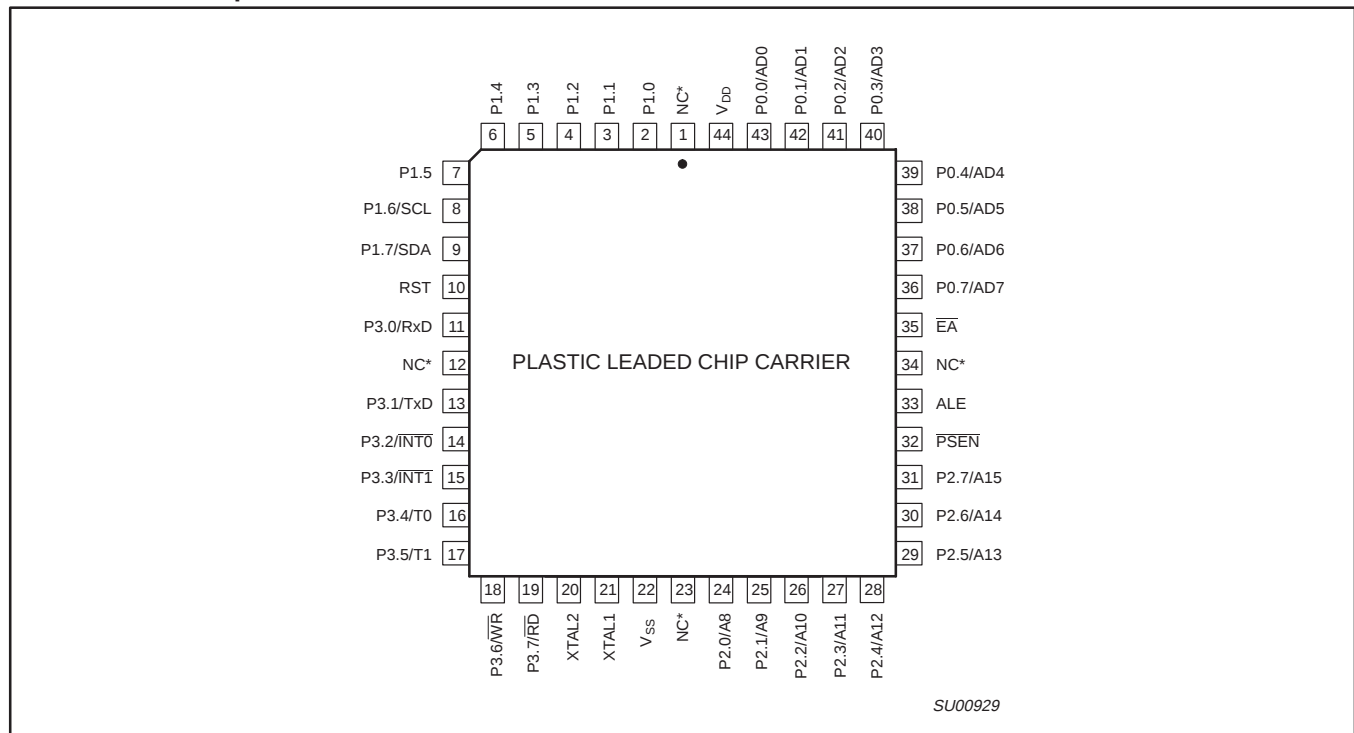
Plastic leaded chip carrier
