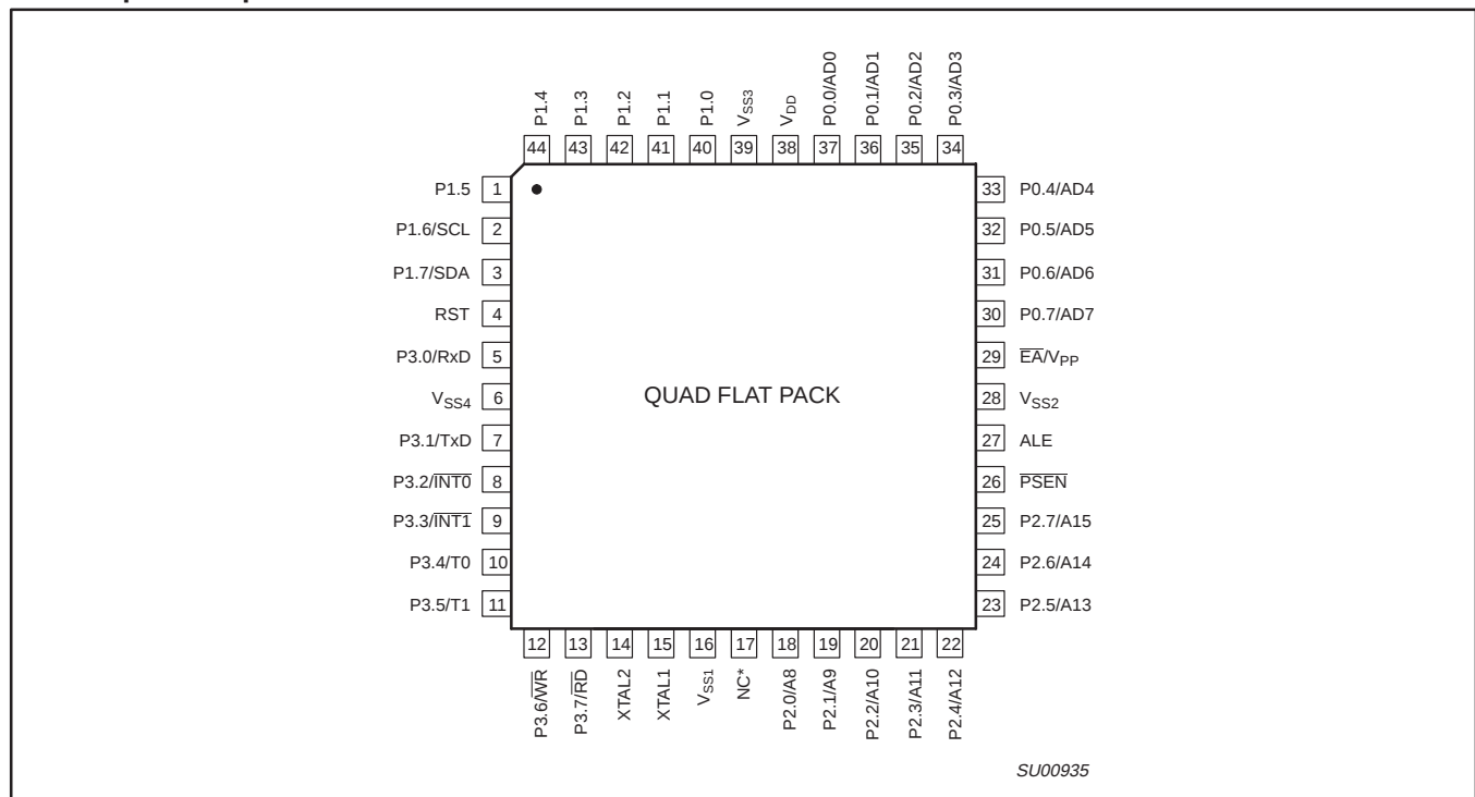
Plastic quad flat pack
