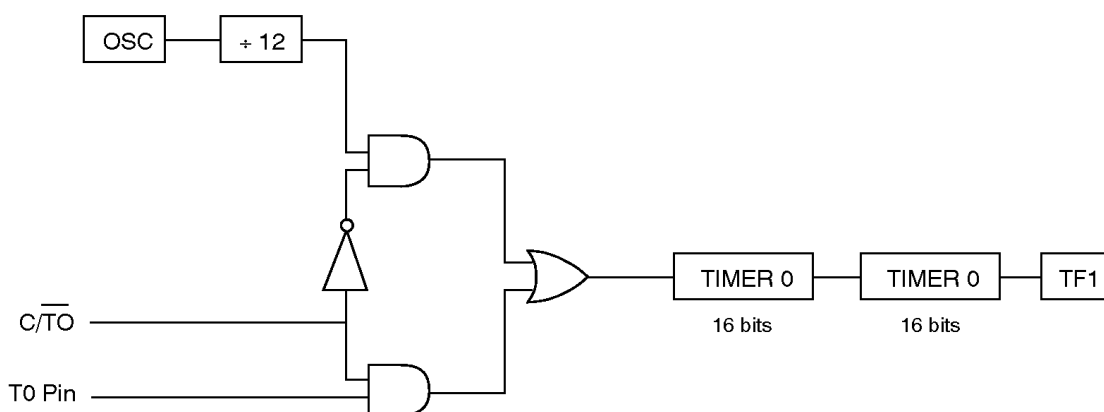
Figure 9. 32 Bit Timer/Counter.
