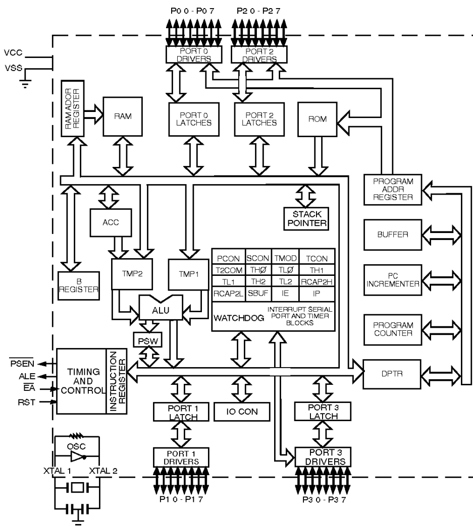
Figure 1. Block Diagram
