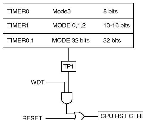
Figure 13. The Different Watchdog Configurations.
