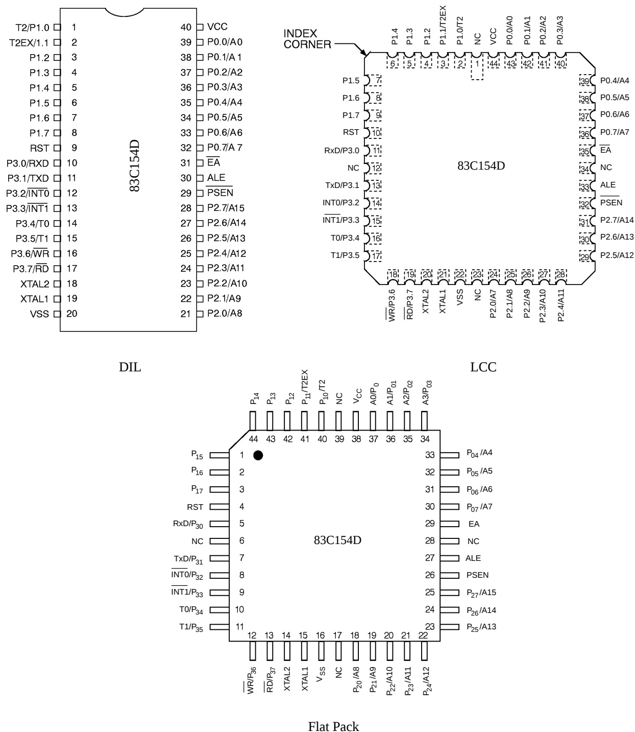
Figure 2. Pin Configuration
