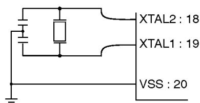
Figure 5. Crystal Oscillator.
