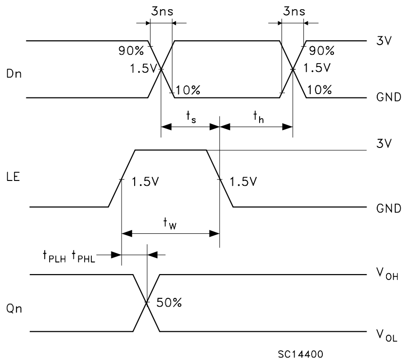
WAVEFORM 1: LE TO Qn PROPAGATION DELAYS, LE MINIMUM PULSE WIDTH, Dn TO LE SETUP AND HOLD TIMES ( f=1\text{MHz} ; 50% duty cycle)
