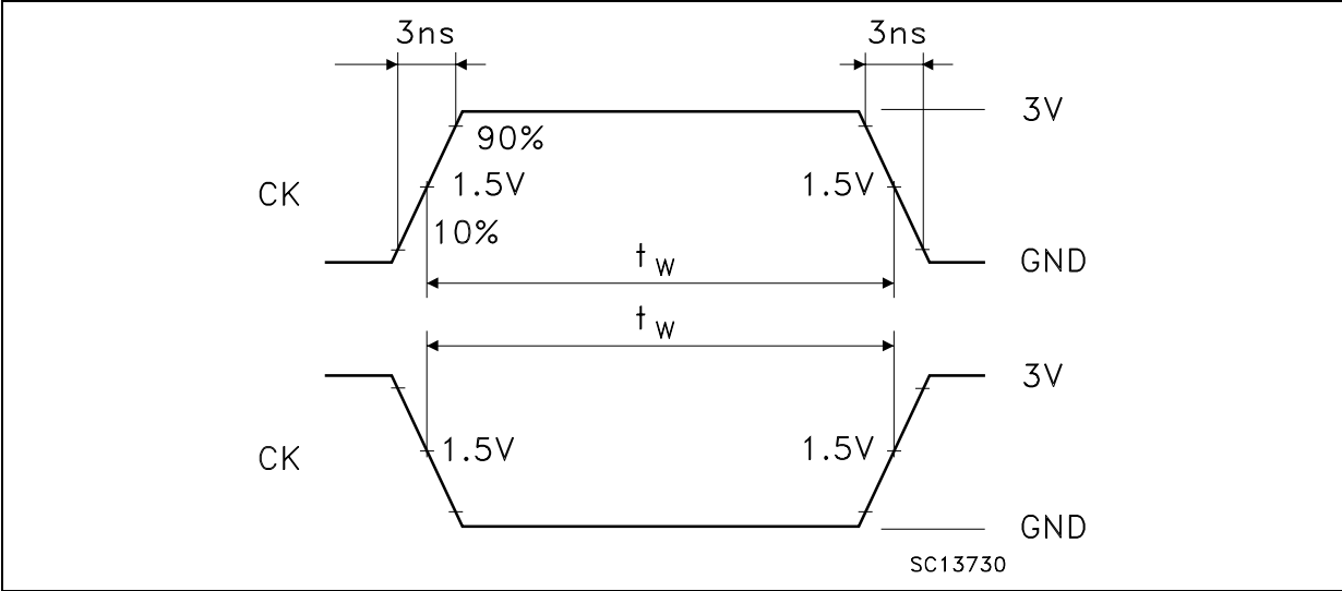
WAVEFORM 3: PULSE WIDTH (f=1MHz; 50% duty cycle)
