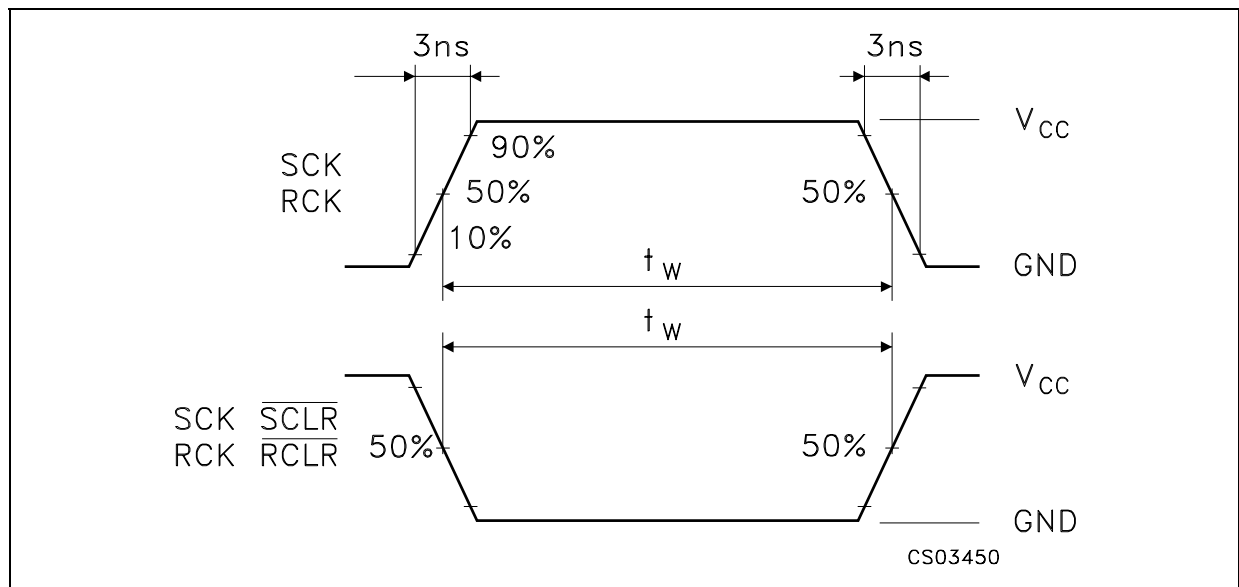
WAVEFORM 2: PULSE WIDTH ( f=1\text{MHz} ; 50% duty cycle)
