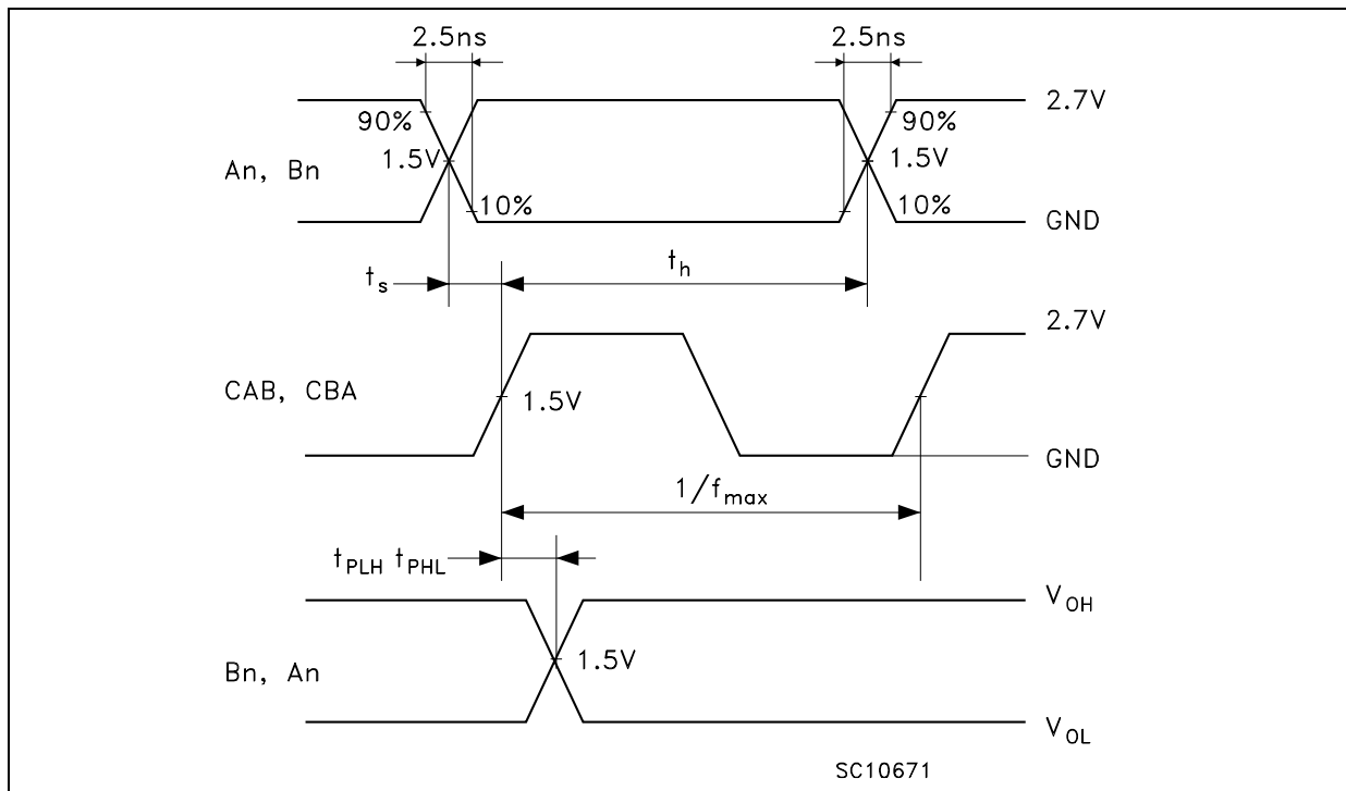
WAVEFORM 3 : SETUP AND HOLD TIME, CAB, CBA MAXIMUM FREQUENCY ( f=1\text{MHz} ; 50% duty cycle)
