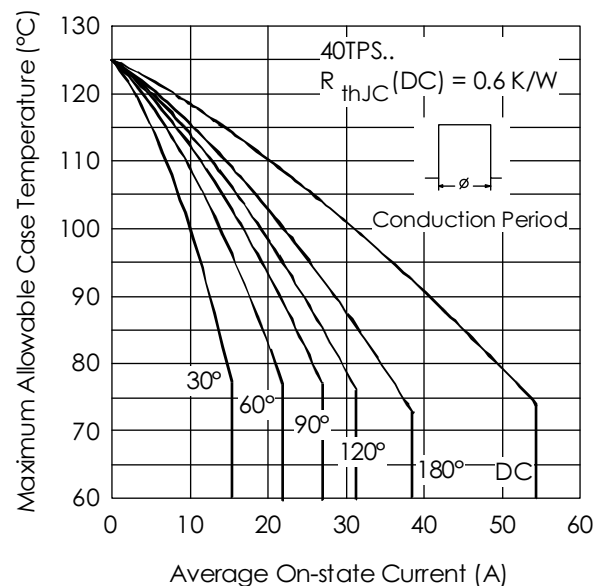
Fig. 2 - Current Rating Characteristics
