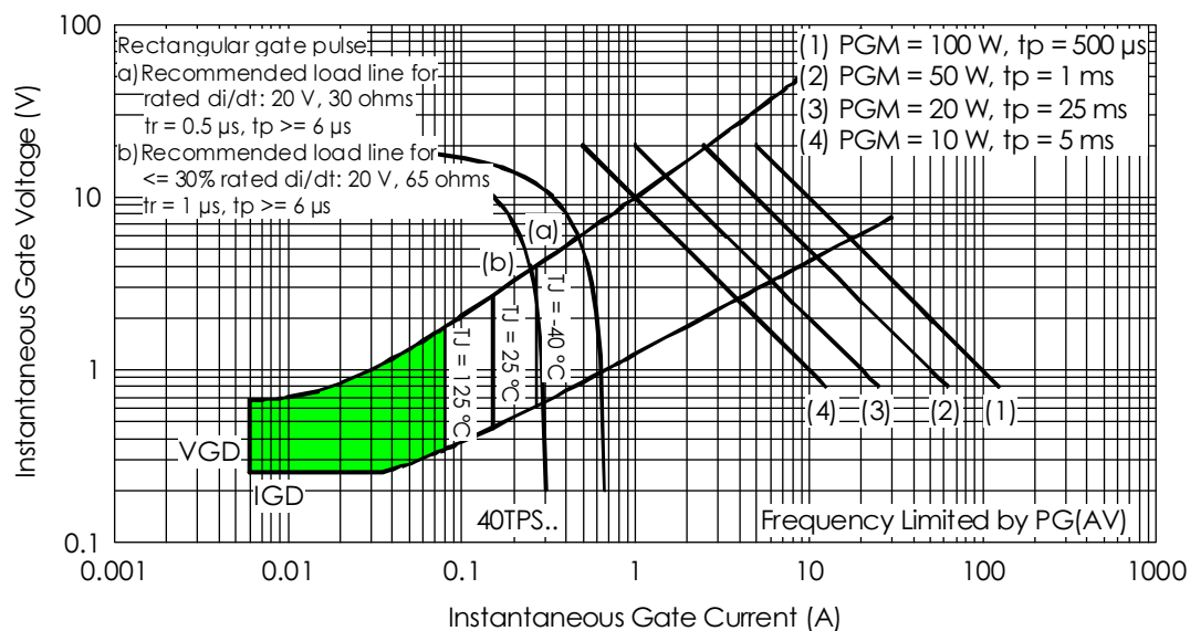
Fig. 8 - Gate Characteristics
