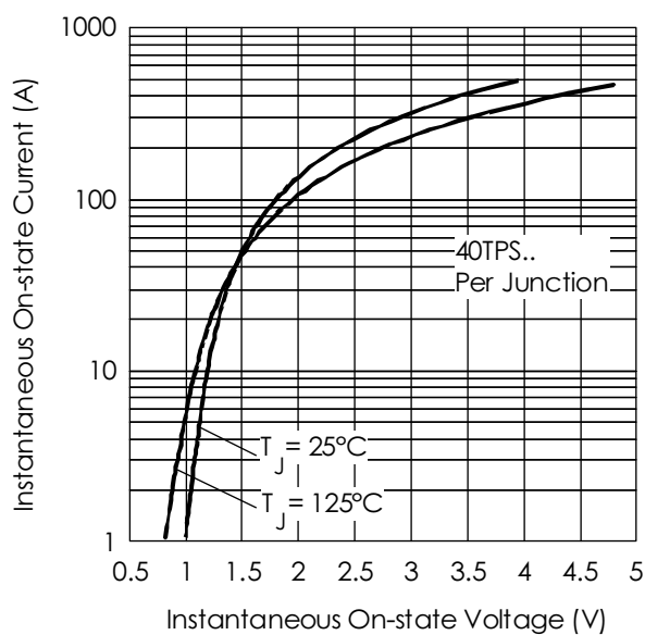
Fig. 7 - On-state Voltage Drop Characteristics
