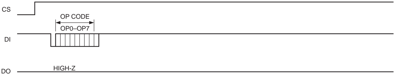
Figure 8. EWEN/EWDS Timing (x8 Format)
