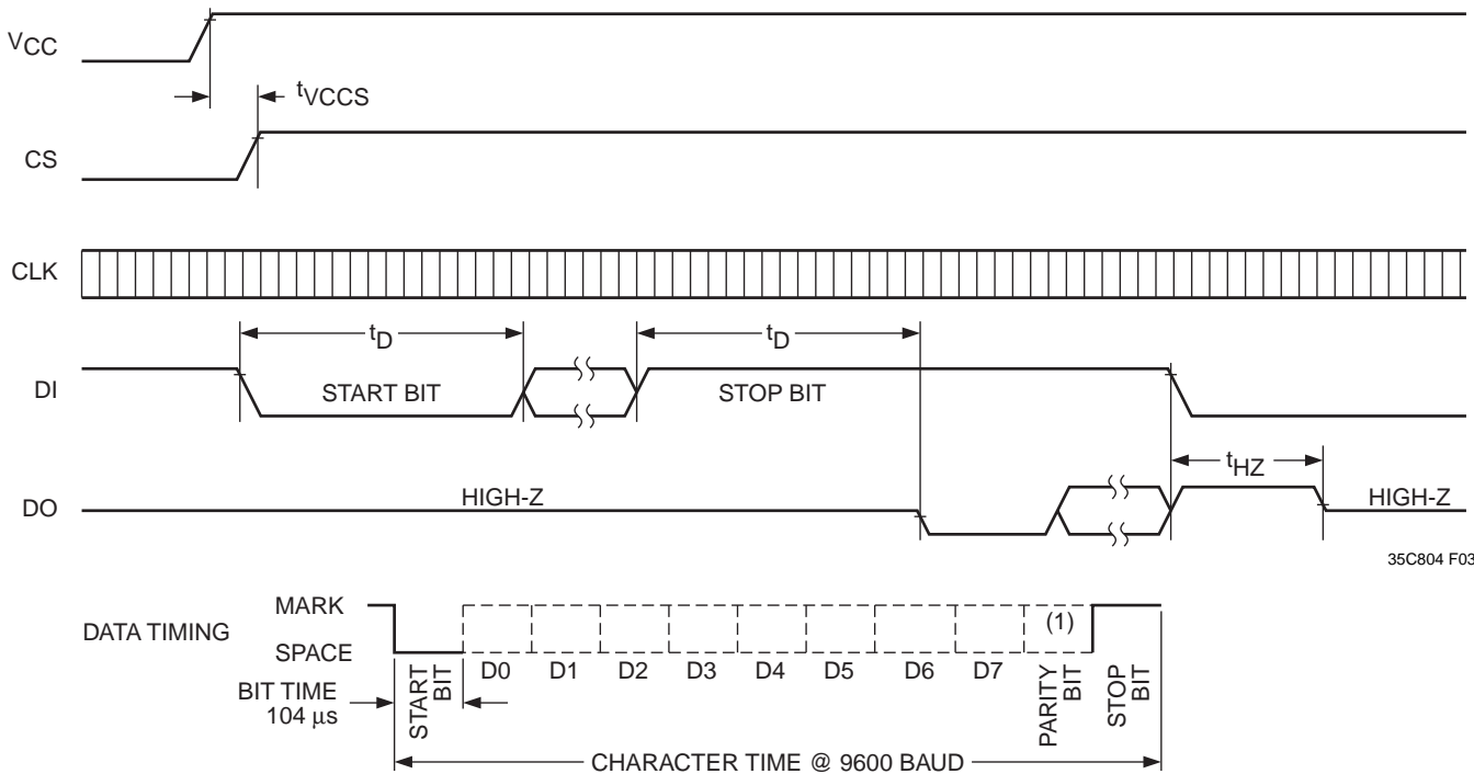
Figure 1. A.C. Timing
