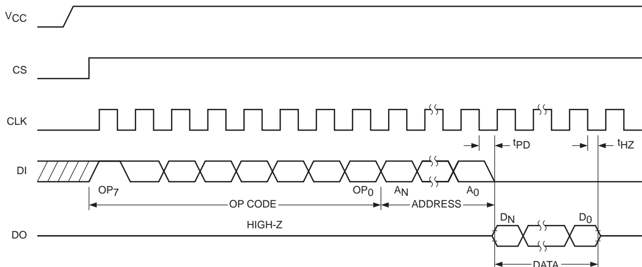
Figure 7. Read Timing
