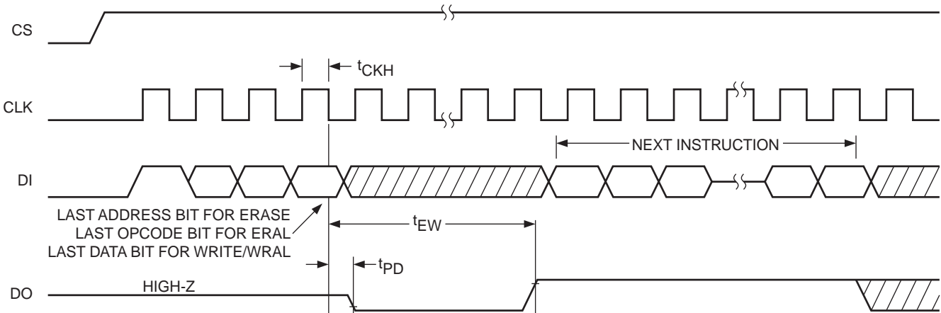
Figure 5. Program/Erase Timing
