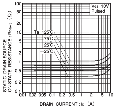
Fig.5 Static drain-source on-resistance vs. drain current
