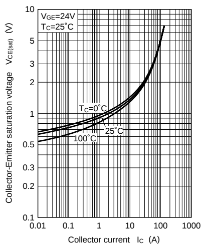
V_{CE(\text{sat})} - I_C
