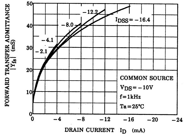
|Yfs| - ID
