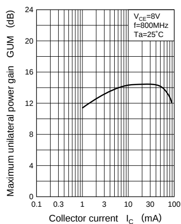
\text{GUM} - I_C
