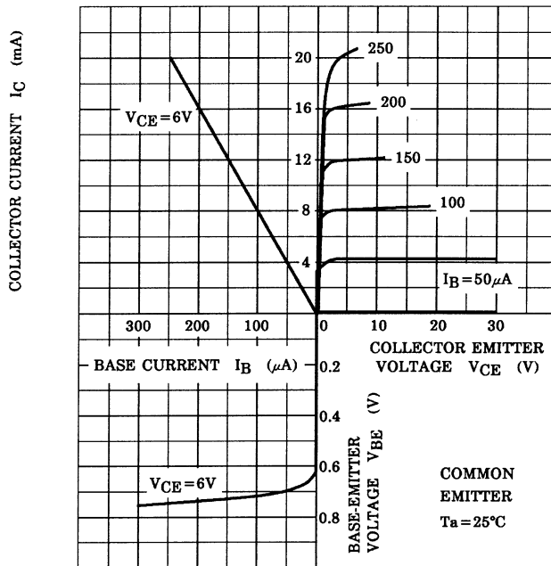
STATIC CHARACTERISTICS
