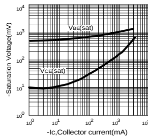
Fig.8 Saturation Voltage
