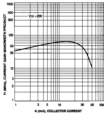
CURRENT GAIN BANDWIDTH PRODUCT
