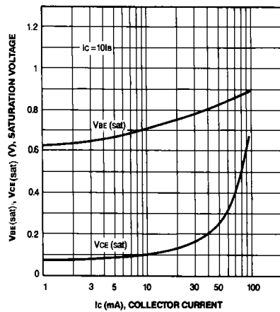
COLLECTOR-EMITTER SATURATION VOLTAGE BASE-EMITTER SATURATION VOLTAGE
