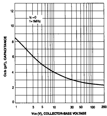
COLLECTOR-BASE CAPACITANCE
