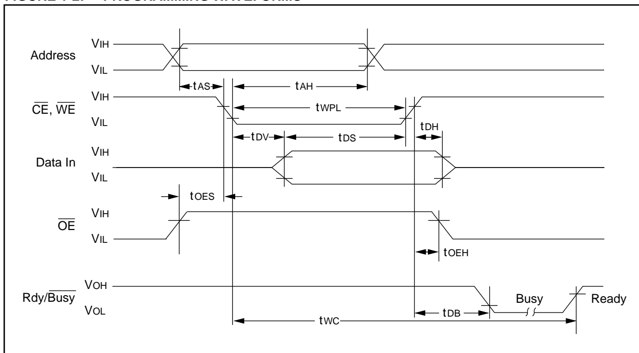
FIGURE 1-2: PROGRAMMING WAVEFORMS
