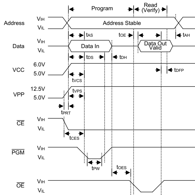
Figure 2. Programming waveforms
