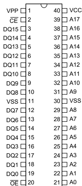
HT27C4096 - 40 DIP-A
