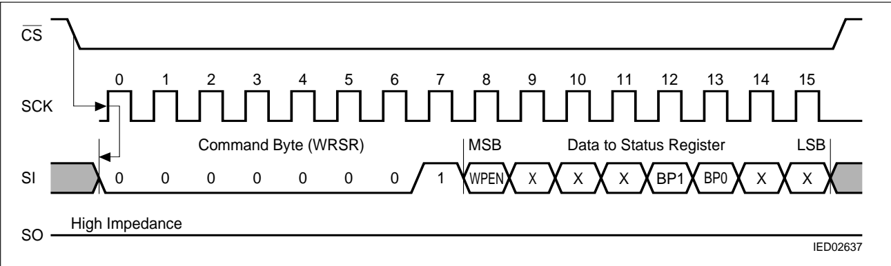
Figure 6 Write to Status Register (WRSR) Sequence
