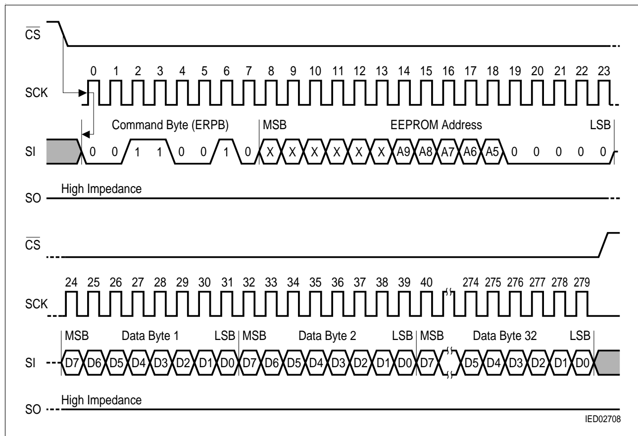
Figure 14 Sequence for Protection Bit Erase
