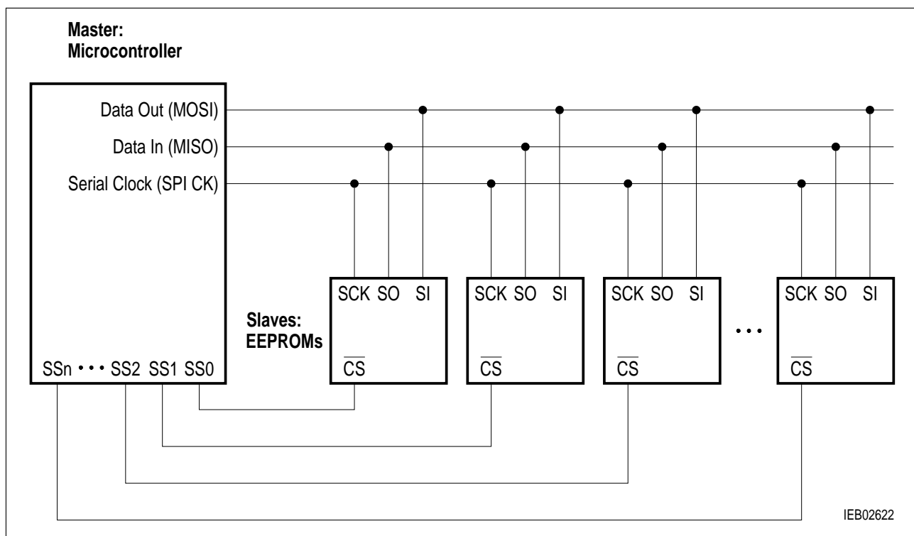
Figure 3 Bus Configuration
