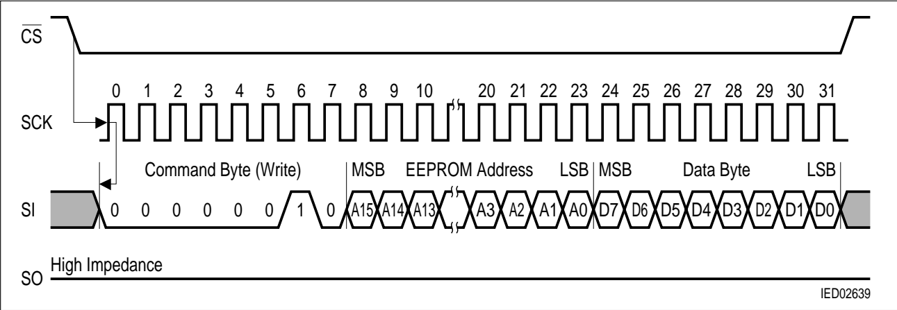
Figure 8 Byte Write Sequence
