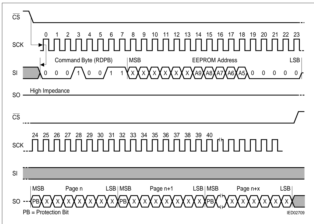
Figure 15 Byte Sequence for Protection Bit Read
