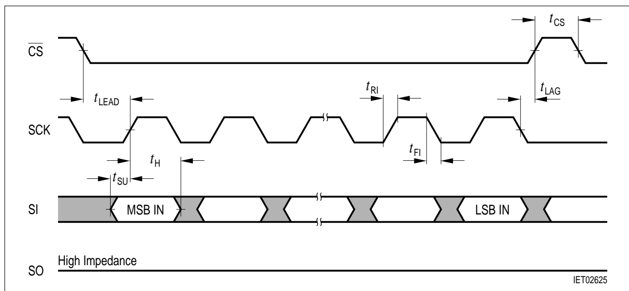
Figure 16 Bus Timing for Serial Input
