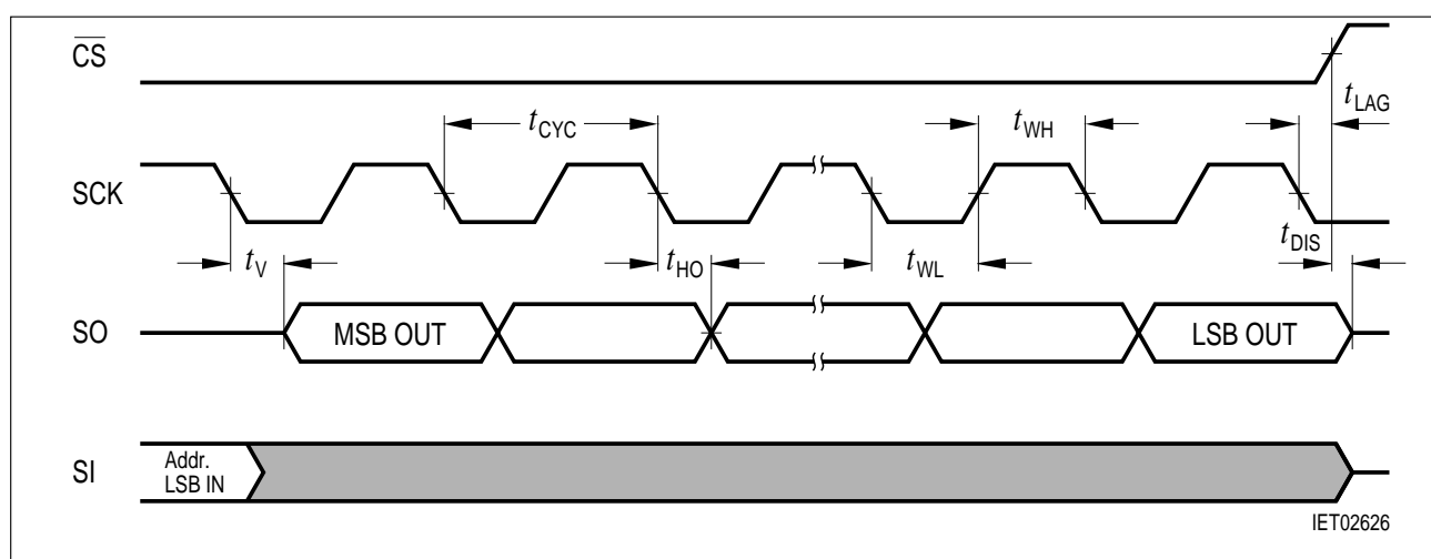
Figure 17 Bus Timing for Serial Output
