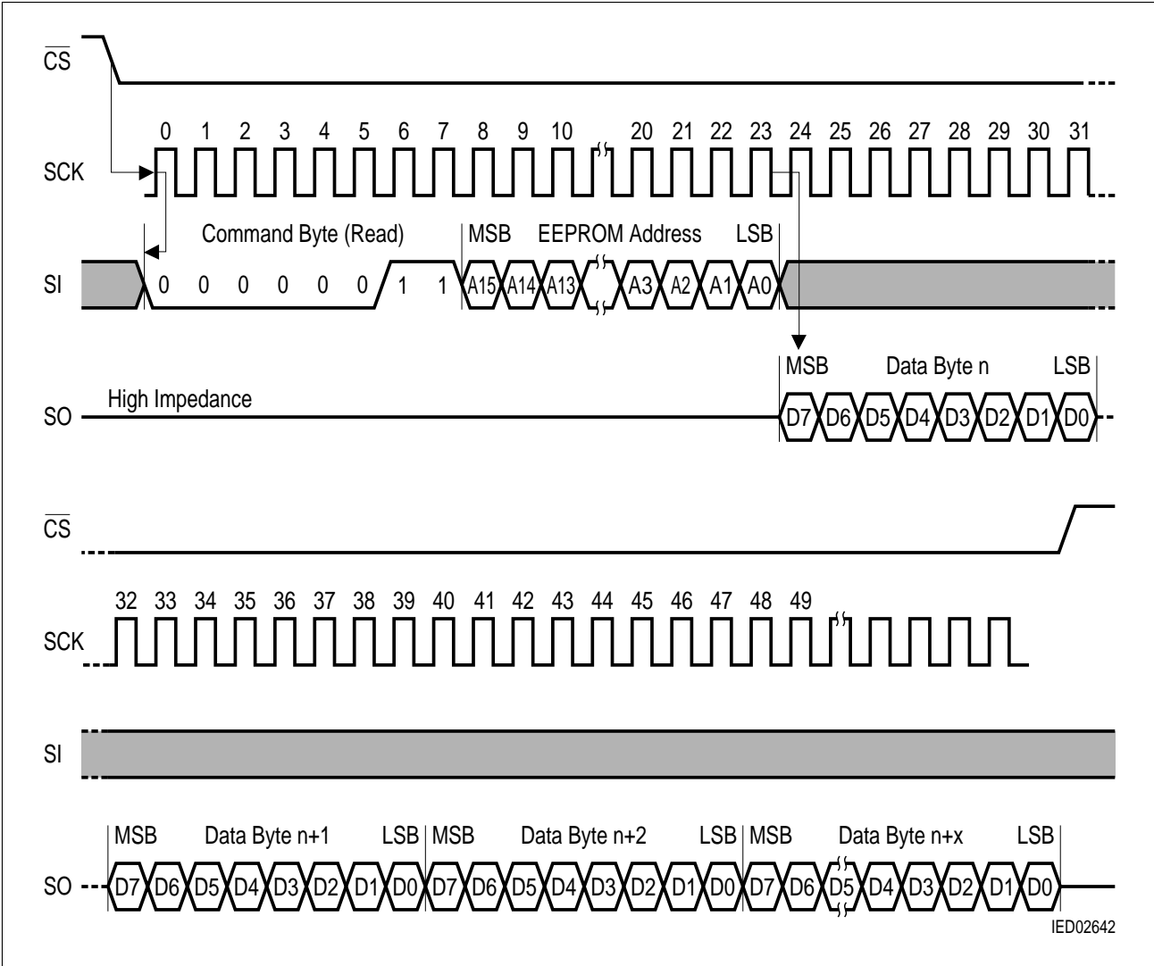
Figure 11 Sequential Read Sequence
