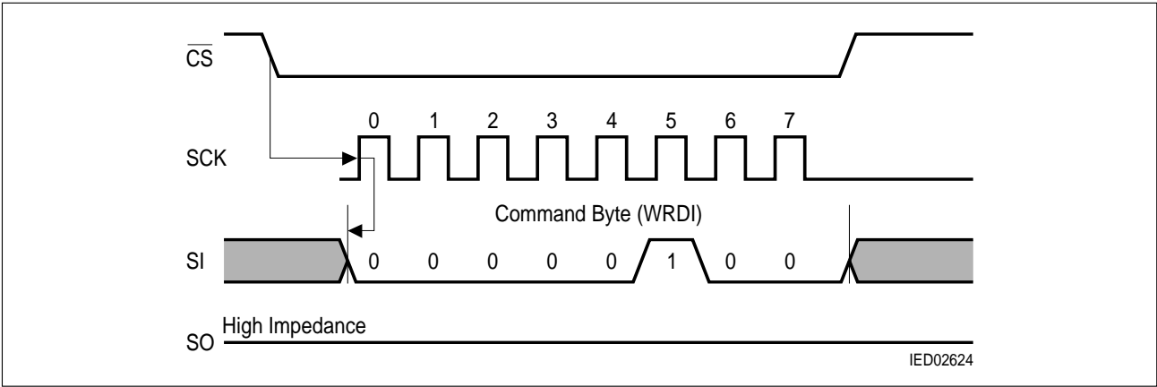
Figure 5 Write Disable (WRDI) Sequence
