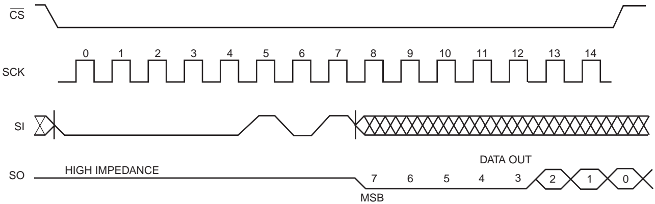
Figure 5. RDSR Timing
