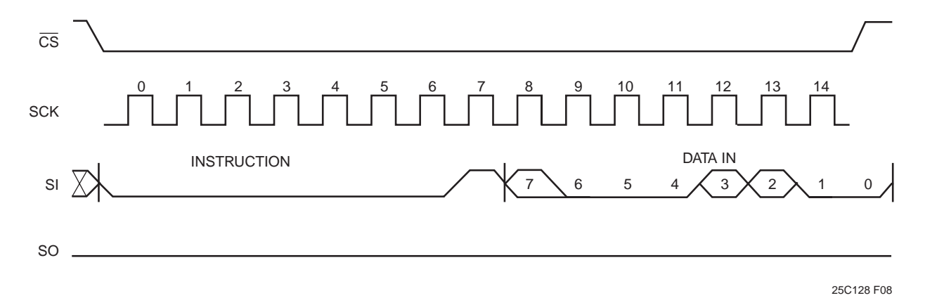
Figure 7. WRSR Timing
