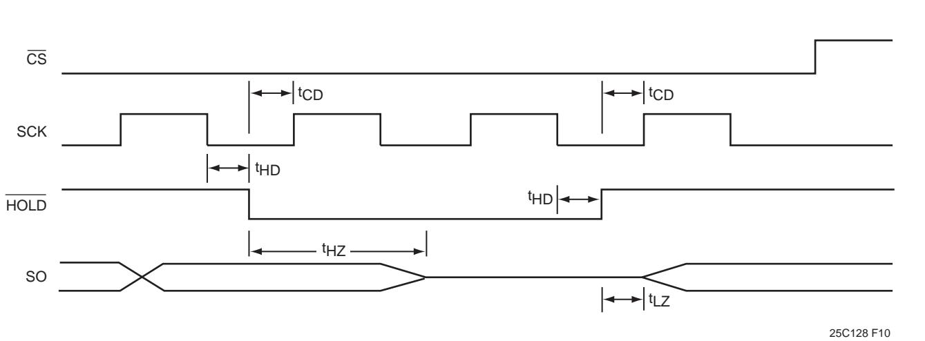
Figure 9. HOLD Timing
