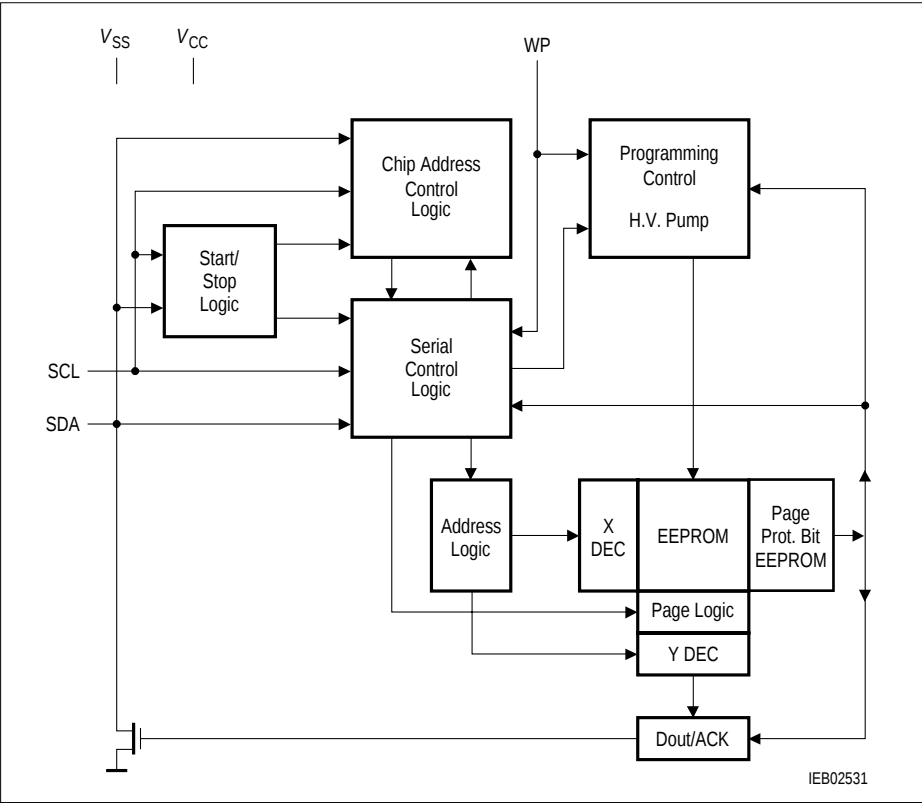
Figure 2 Block Diagram
