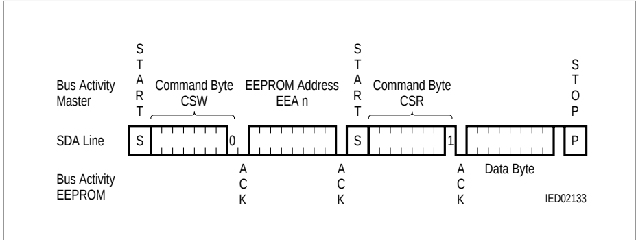
Figure 11 Random Read
