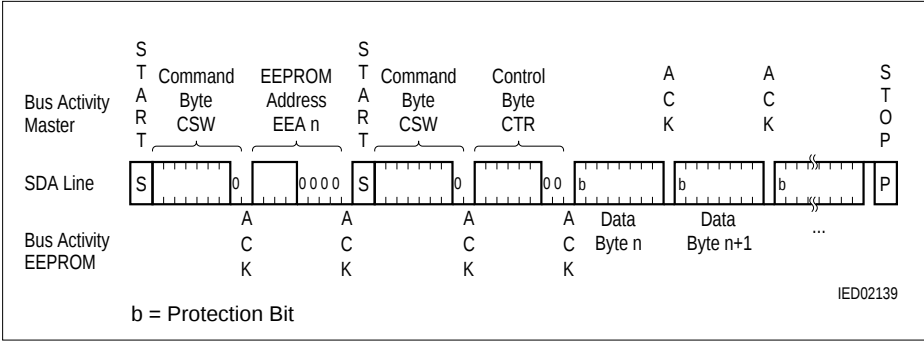
Figure 17 Byte Sequence for Protection Bit Read
