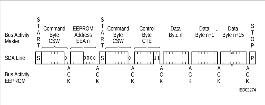
Figure 16 Sequence for Protection Bit Erase
