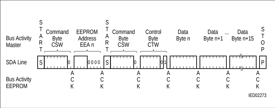
Figure 15 Sequence for Protection Bit Write
