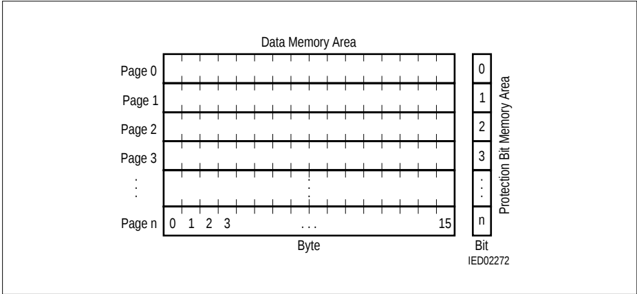
Figure 14 Data Page and Assigned Protection Memory
