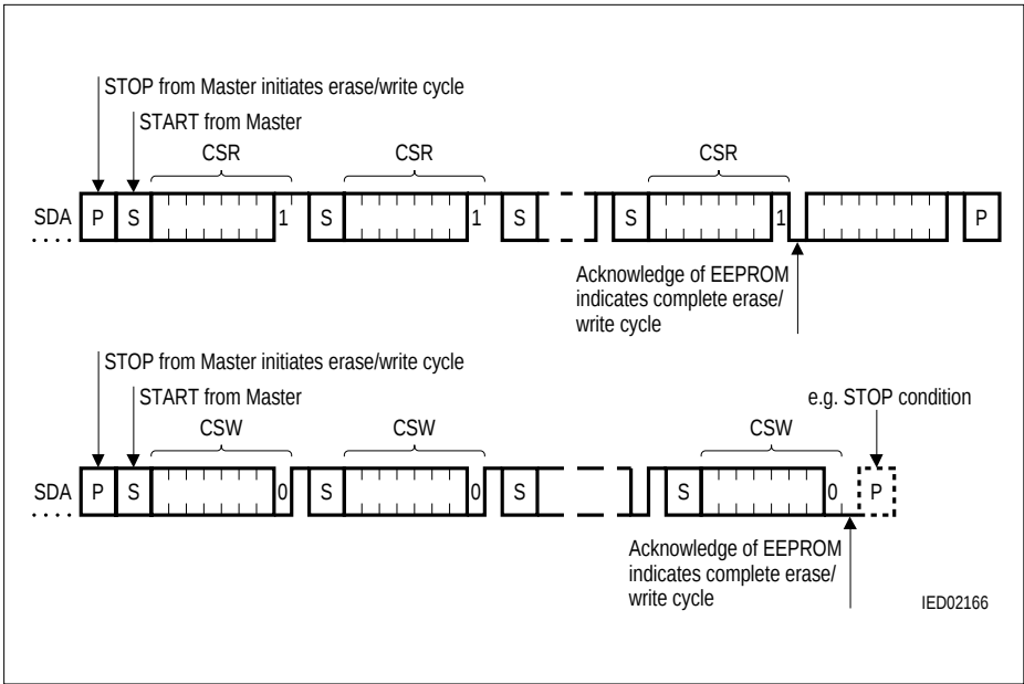
Figure 10 Principle of Acknowledge Polling
