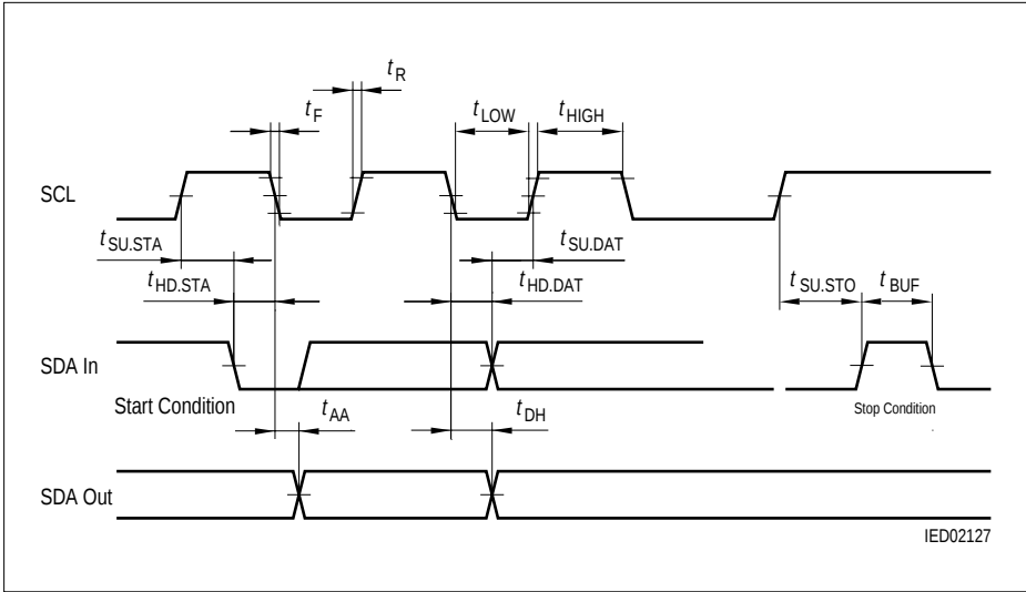
Figure 18 Bus Timing Data
