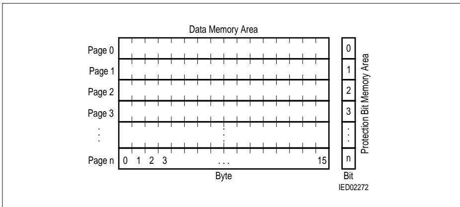
Figure 14 Data Page and Assigned Protection Memory
