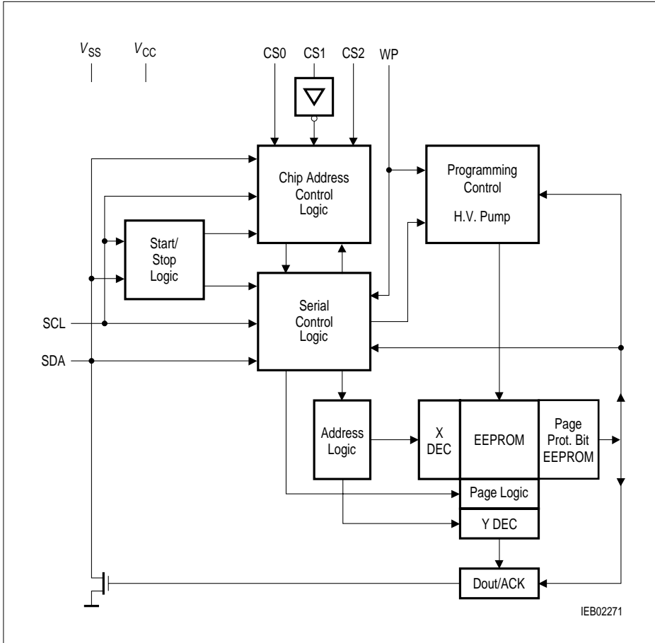
Figure 2 Block Diagram
