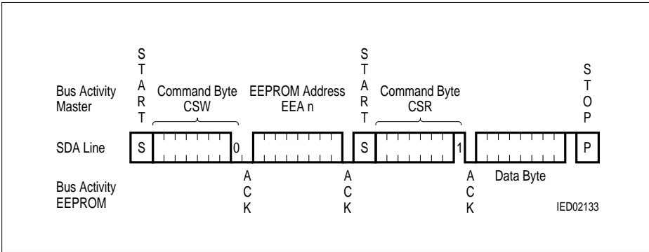
Figure 11 Random Read
