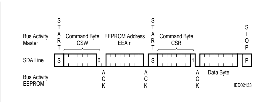
Figure 11 Random Read
