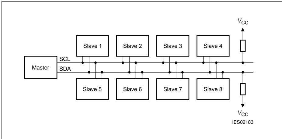
Figure 3 Bus Configuration
