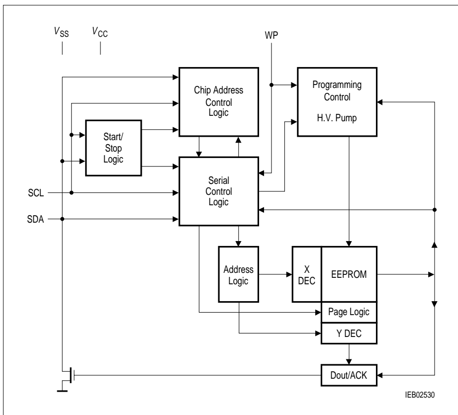
Figure 2 Block Diagram
