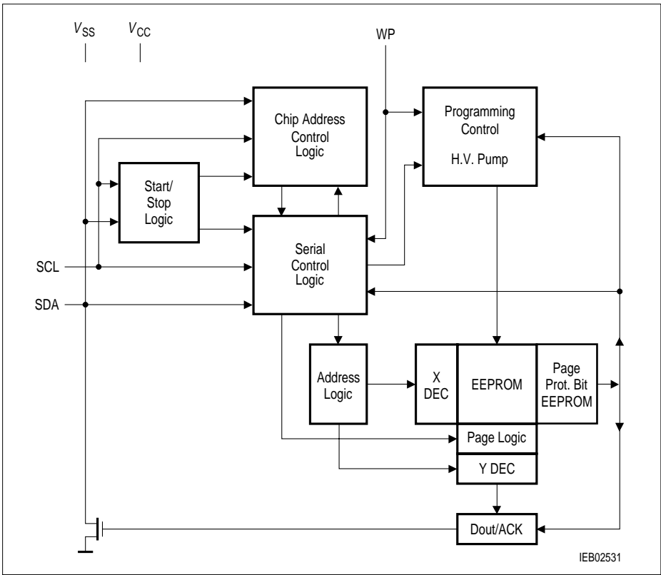
Figure 2 Block Diagram
