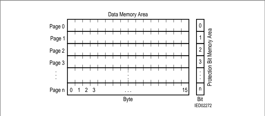
Figure 14 Data Page and Assigned Protection Memory
