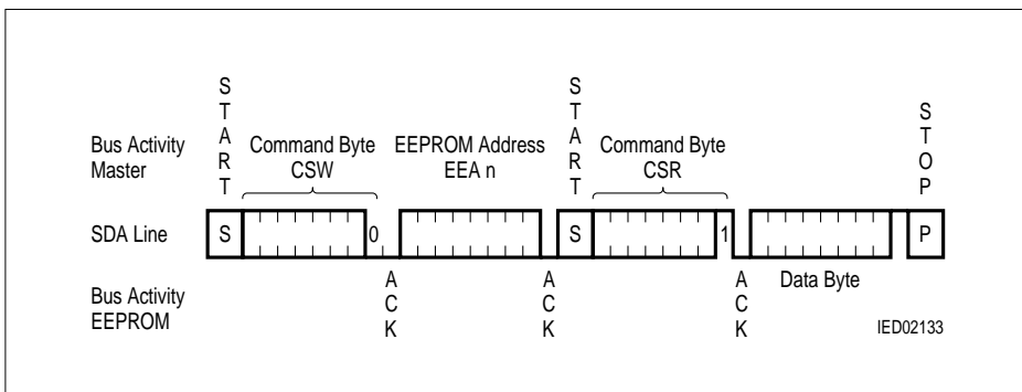
Figure 11 Random Read
